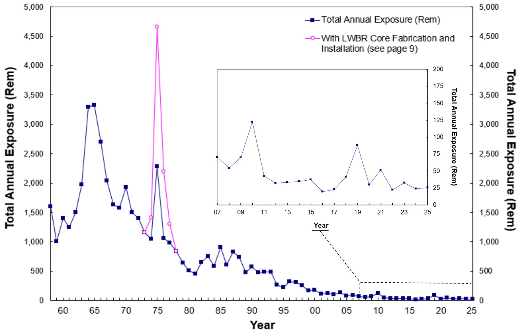
FIGURE 1 TOTAL RADIATION EXPOSURE RECEIVED BY PERSONNEL AT NAVAL REACTORS' DEPARTMENT OF ENERGY FACILITIES 1958 - 2025
