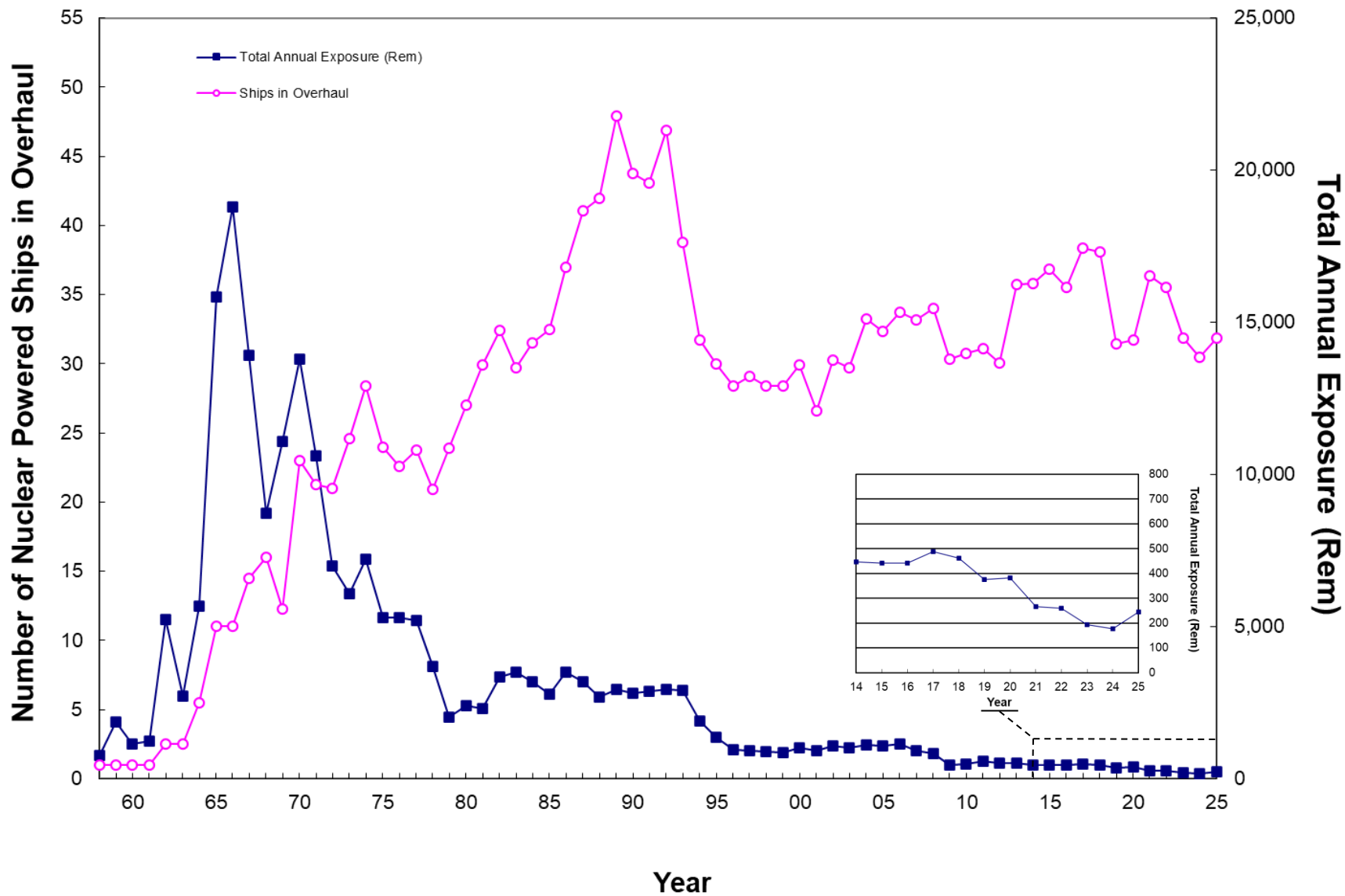
FIGURE 2 TOTAL RADIATION EXPOSURE RECEIVED BY SHIPYARD PERSONNEL FROM WORK ON NAVAL NUCLEAR PROPULSION PLANTS 1958 - 2025
