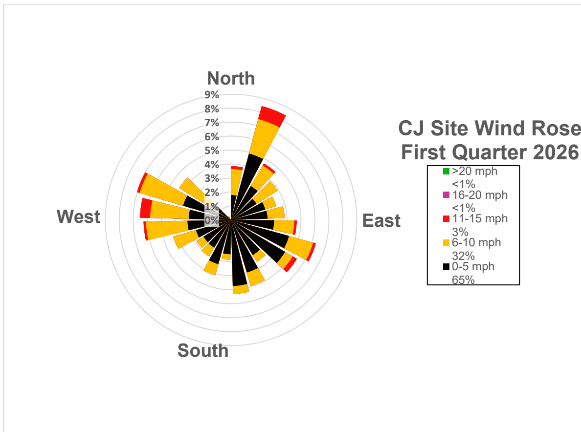
Figure 4. Crescent Junction Wind Rose for First Quarter 2026
