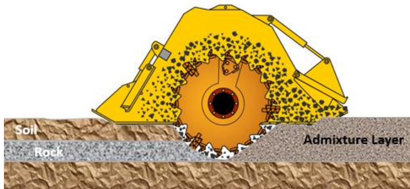
Figure 2 - Rock/Soil Placement
