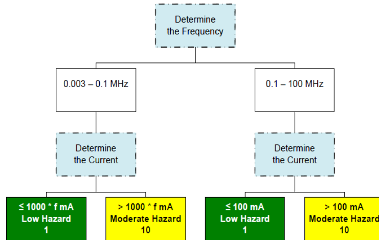
Chart 7. RF circuits, 3 kHz to 100 MHz.
