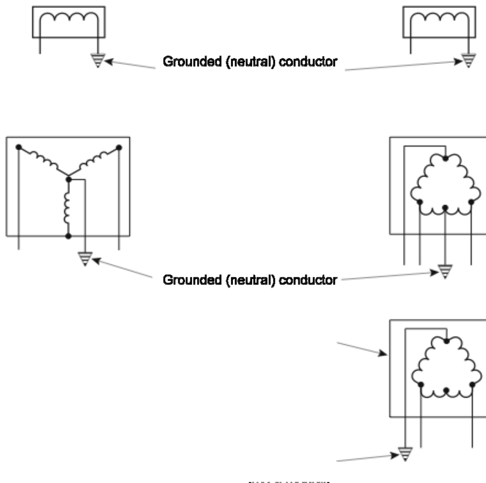
Fig. 5-5. Grounding for systems of 50 to 1,000 V AC.
