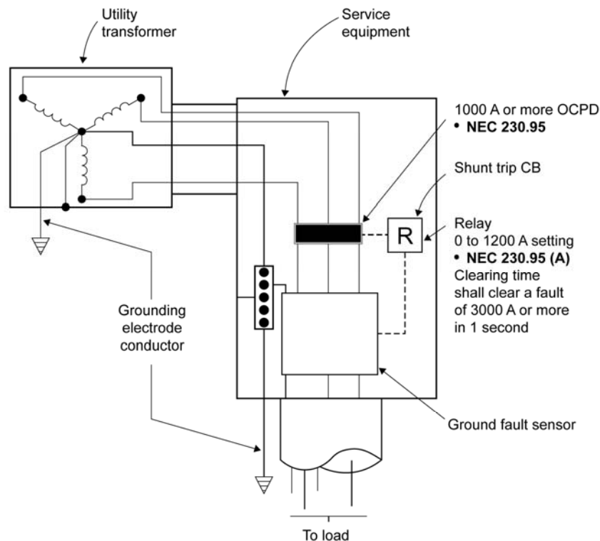
Fig. 4-2. Example of ground fault protection of equipment.
