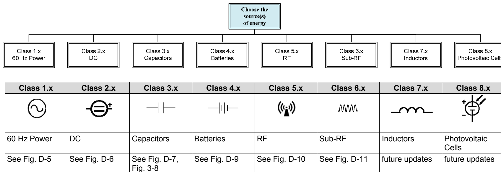
Fig. D-4. Complete Electrical Hazard Classification System Showing Eight Major Groups and 53 Classes.
