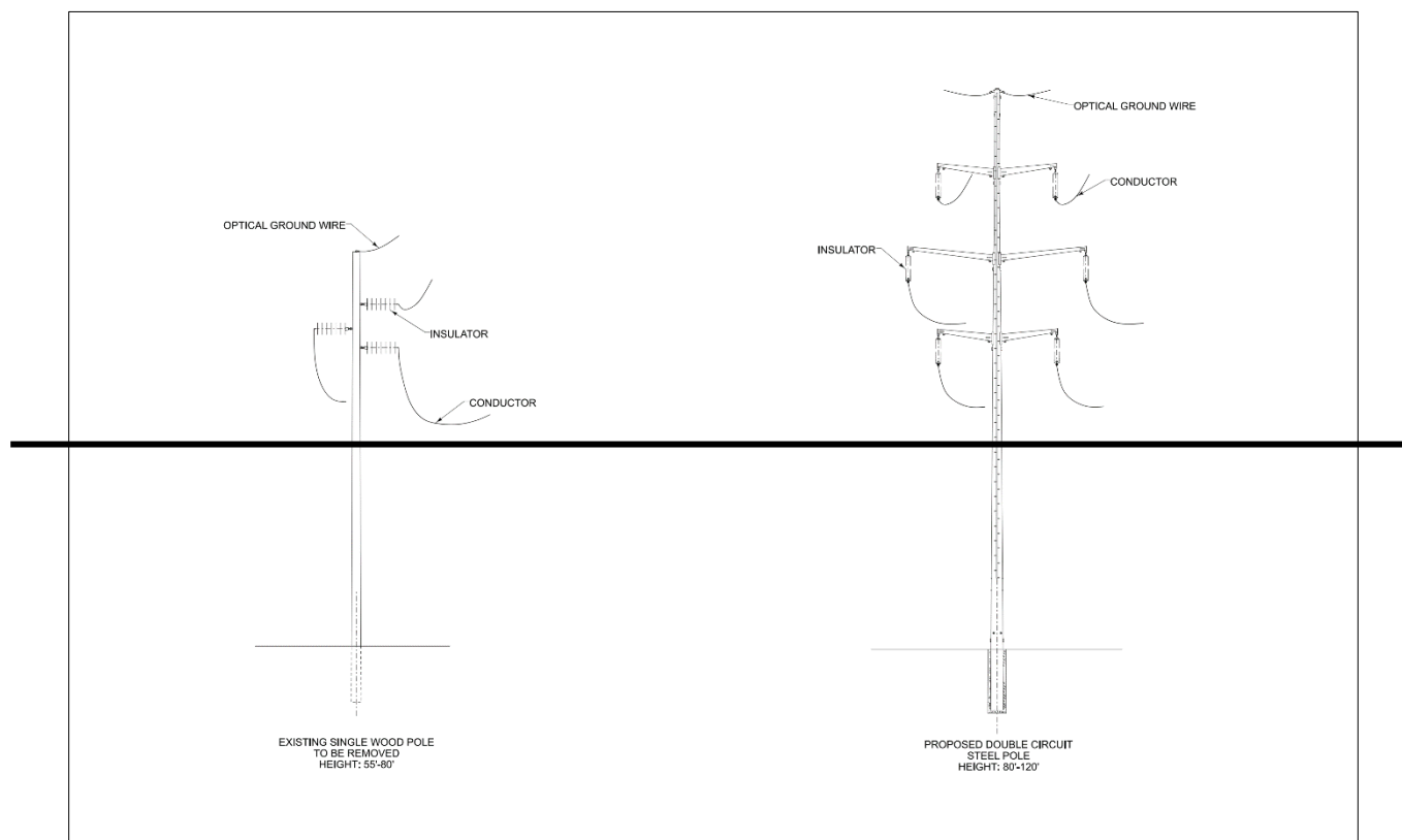
Figure 2-3: Webber Canyon-Badger Canyon Double-Circuit Transmission Structures
