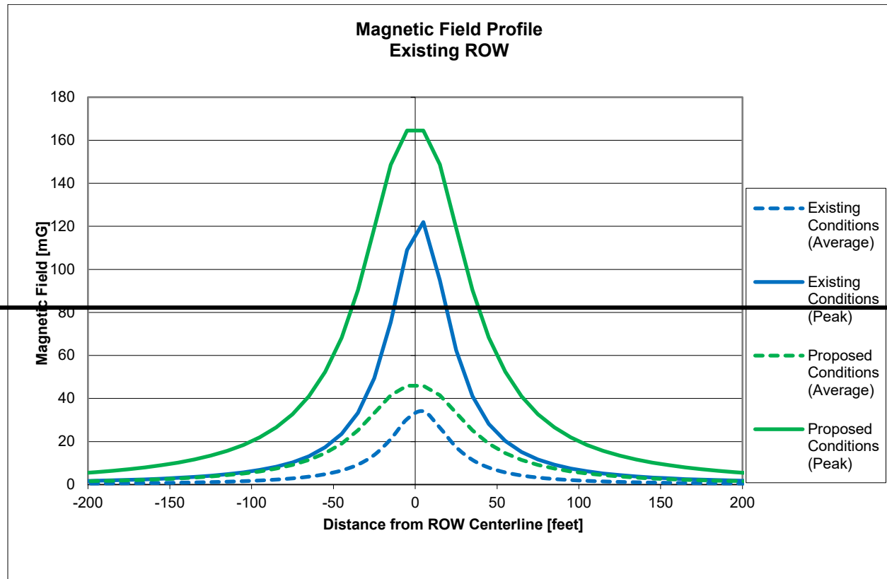
Figure 3-2: Webber Canyon-Badger Canyon Transmission Line Magnetic Field Values (mG) along Existing ROW (Double-Circuit Portion)
