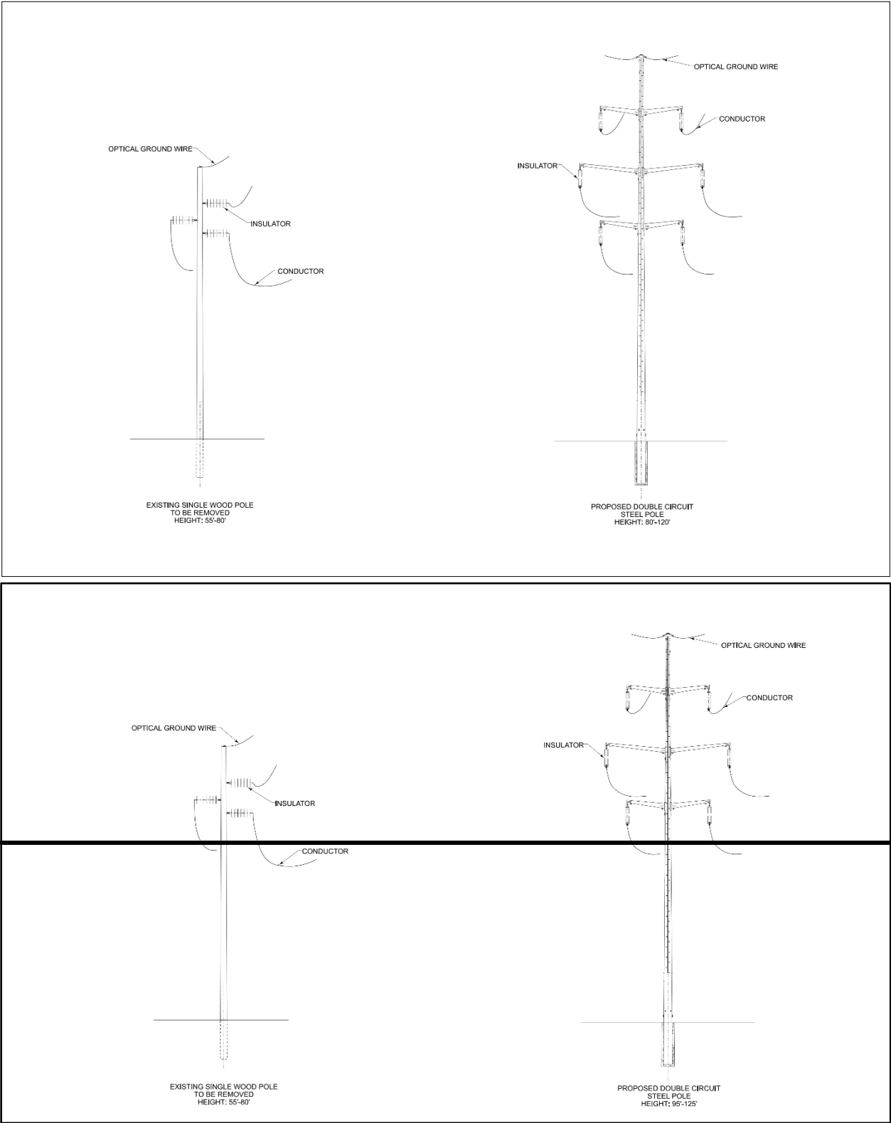
Figure 2-5: Webber Canyon-Badger Canyon Double-Circuit Transmission Structures
