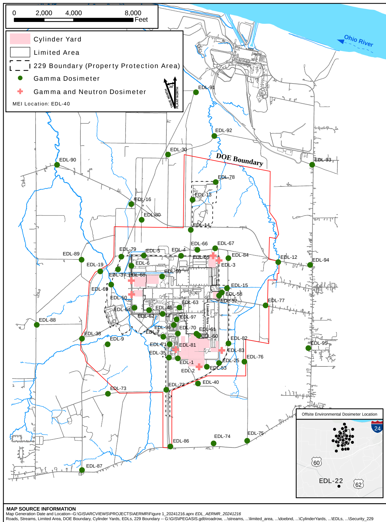
Figure 4.4. Environmental dosimeter locations
