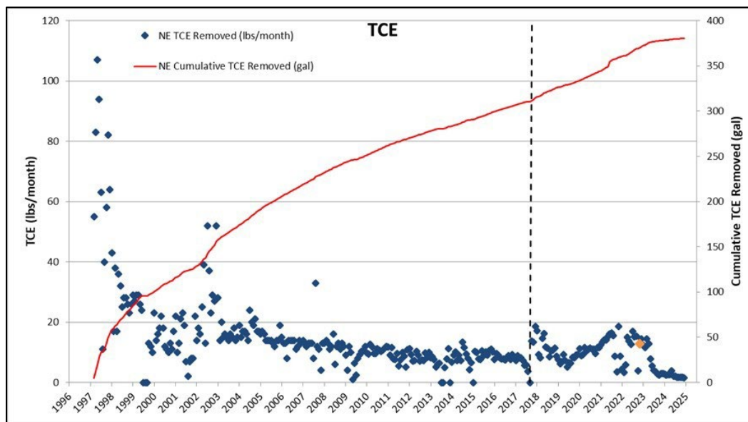
Figure 6.3. Northwest Plume groundwater treatment system trichloroethene removed
