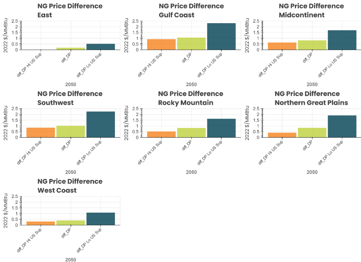
Figure 6. Differences in regional natural gas prices between Model Resolved and Existing/FID Exports scenarios in 2050 for each supply assumption
