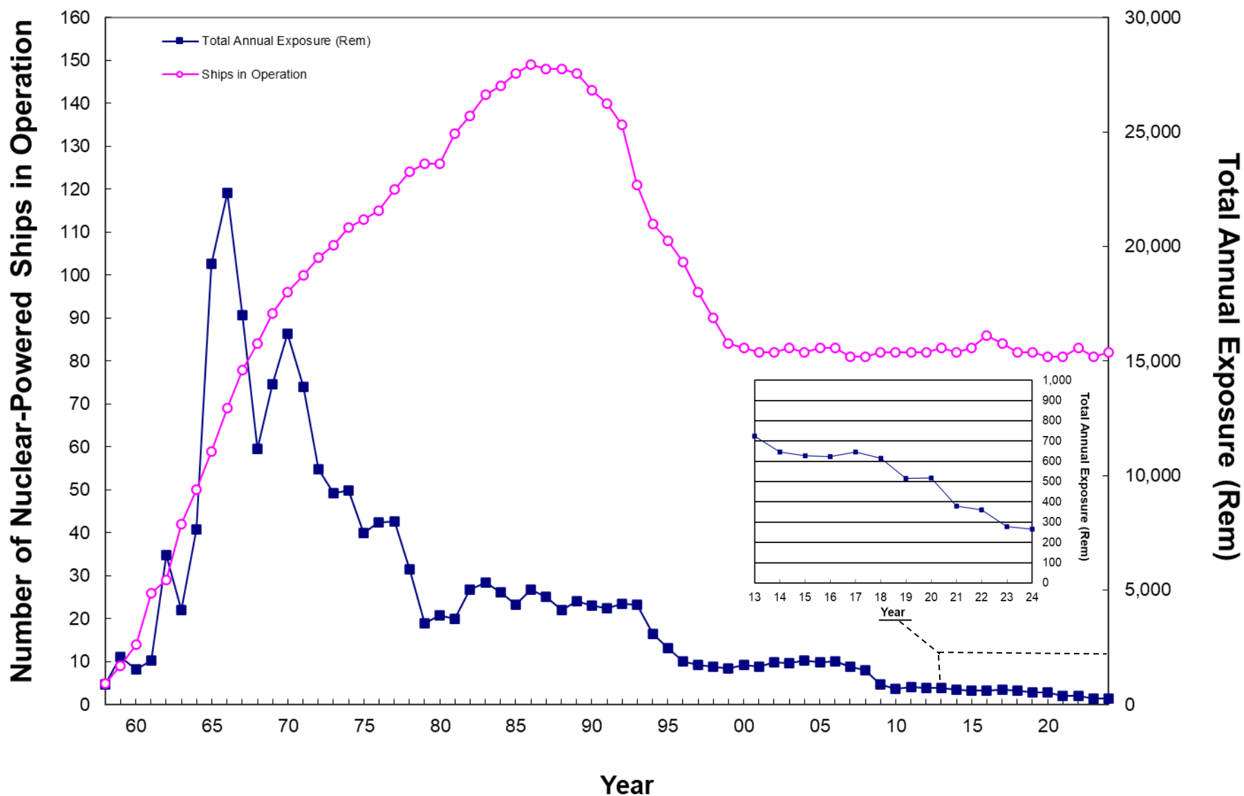
FIGURE 1 TOTAL RADIATION EXPOSURE RECEIVED BY MILITARY AND CIVILIAN PERSONNEL IN THE NAVAL NUCLEAR PROPULSION PROGRAM 1958 - 2024
