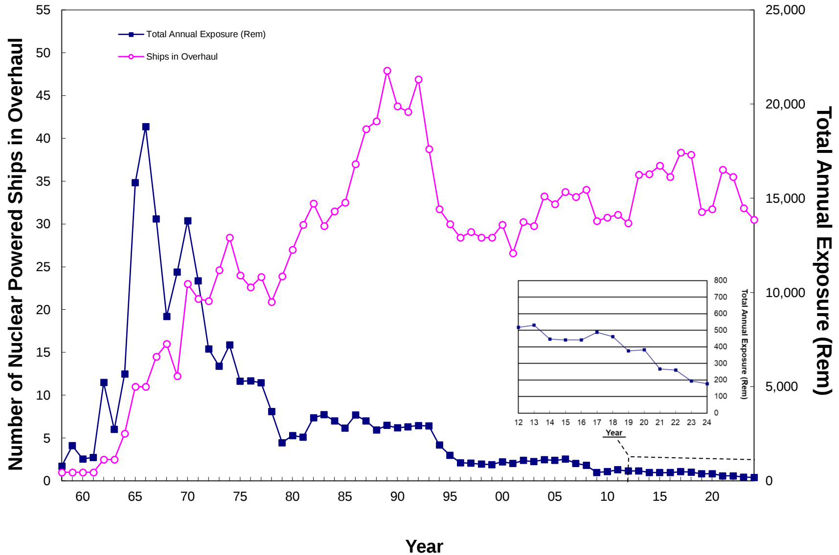
FIGURE 2 TOTAL RADIATION EXPOSURE RECEIVED BY SHIPYARD PERSONNEL FROM WORK ON NAVAL NUCLEAR PROPULSION PLANTS 1958 - 2024
