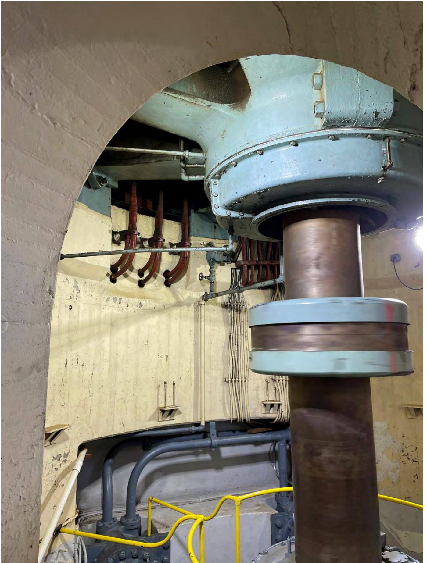
Figure 5. Photograph showing turbine detail.
