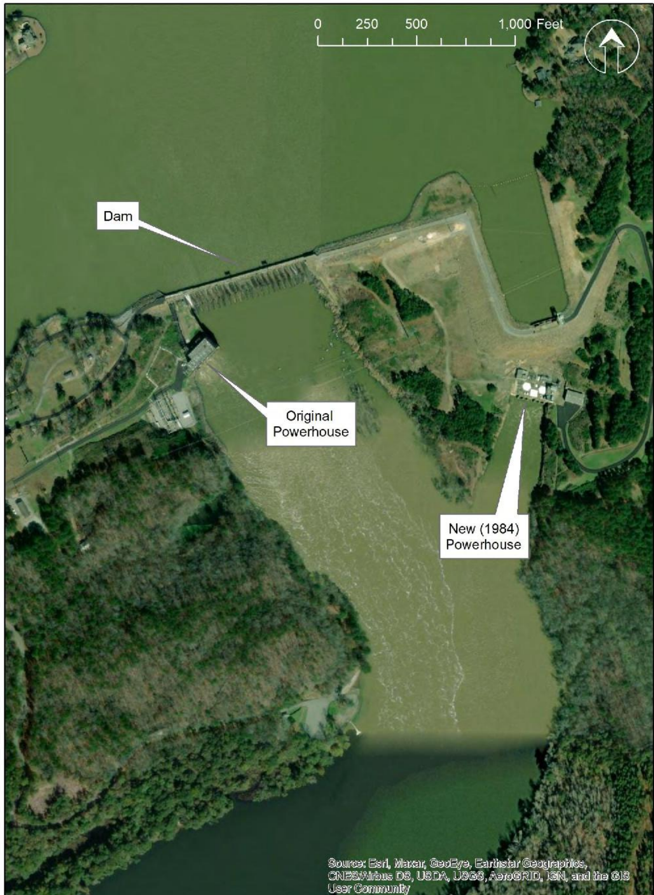
Figure 2. Aerial photograph of Bartletts Ferry project works.
