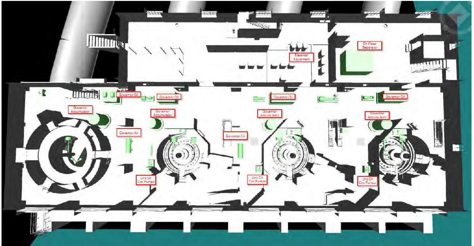
Figure 8. Model of turbine floor before modernization.
