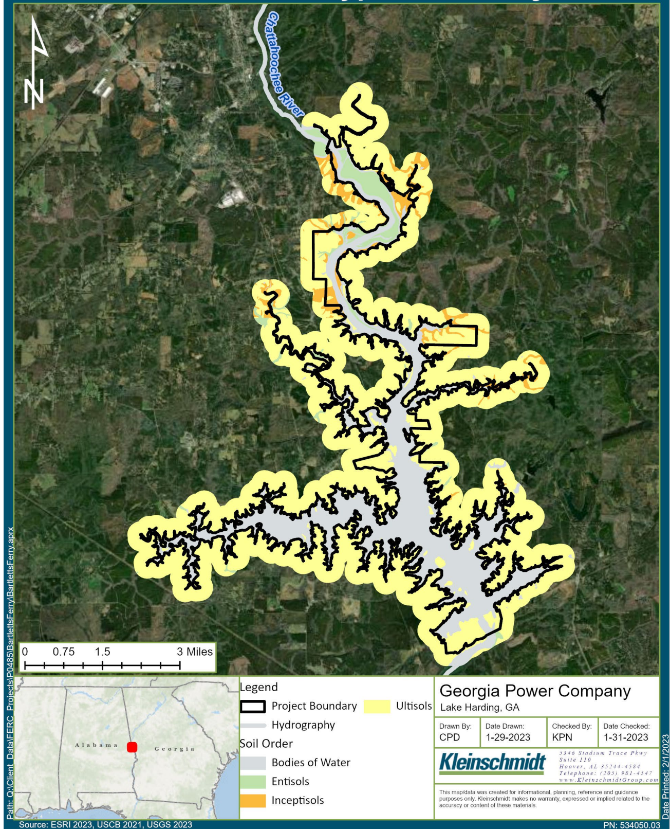
Figure 5-1 Soil Types at the Bartletts Ferry Project
