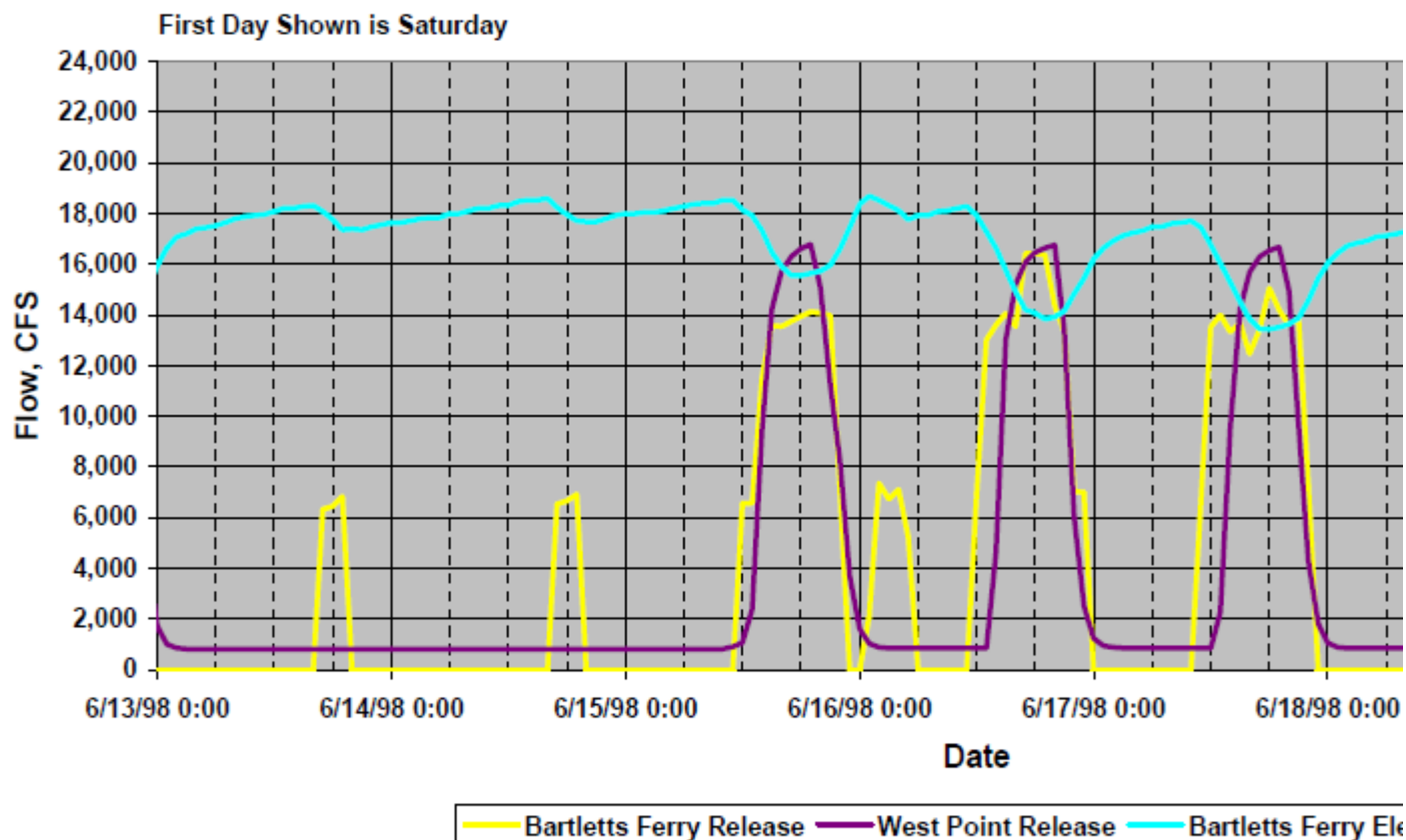
Bartletts Ferry Example of One Week of Operation Medium Inflow (4,742 CFS Average Inflow) With No Weekend West Point Peaking
