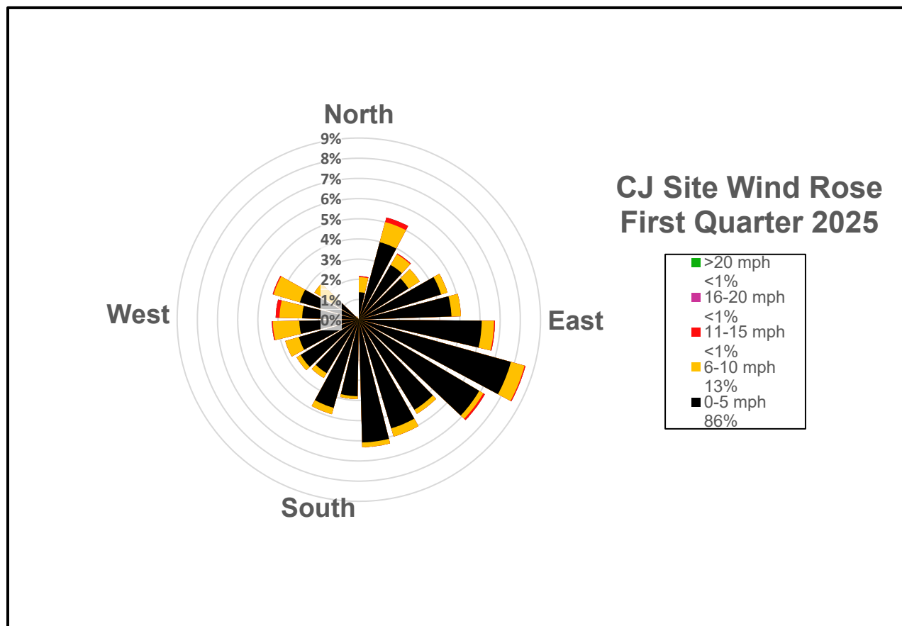
Figure 5. Crescent Junction Wind Rose for First Quarter 2025
