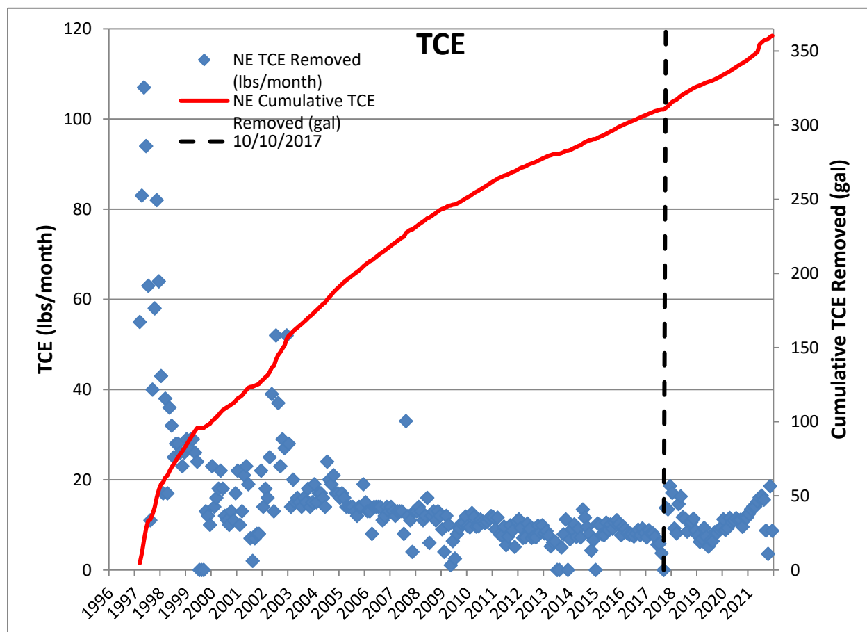
Figure 6.4. Northeast Plume containment system trichloroethene removed
