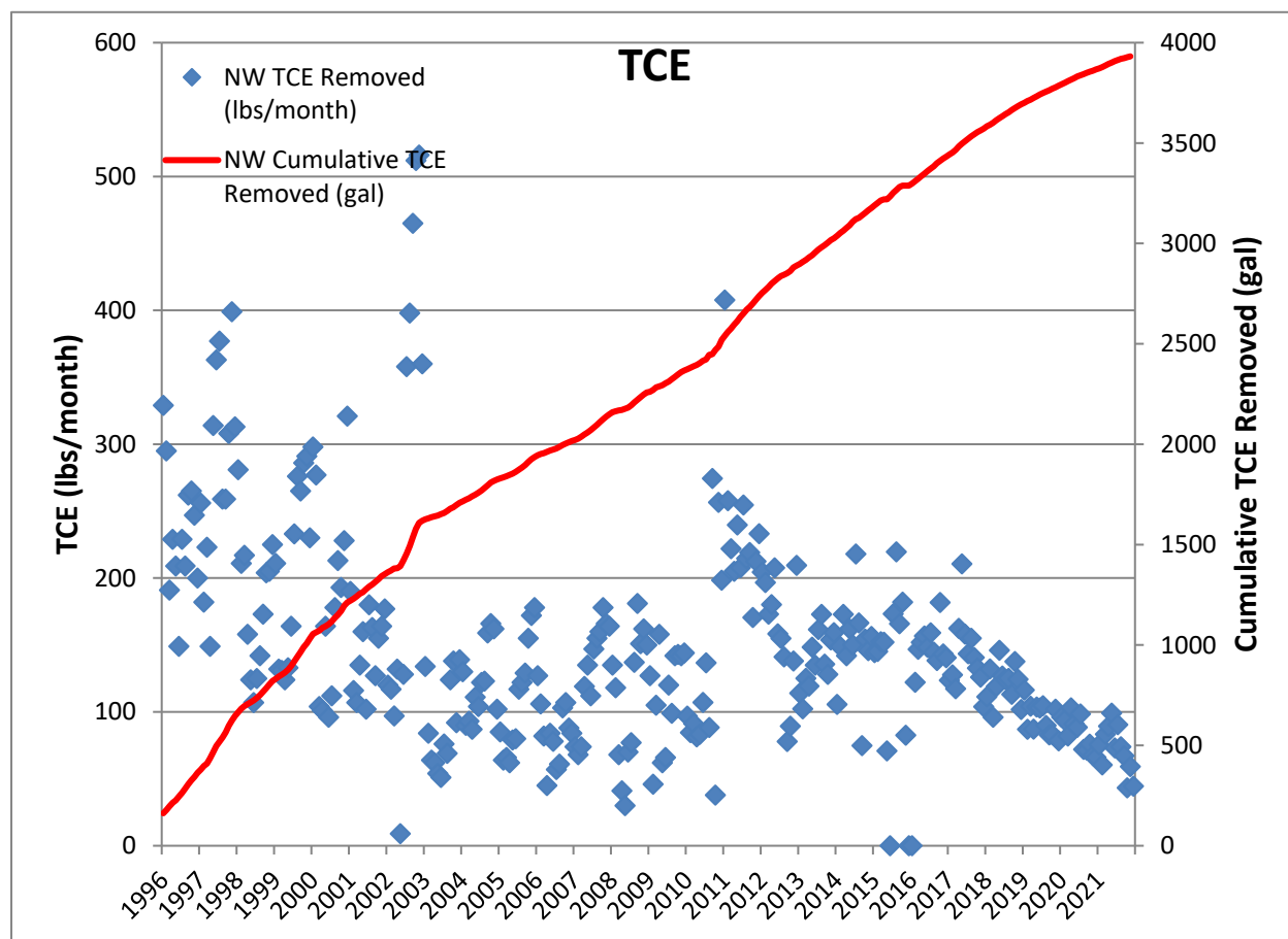
Figure 6.3. Northwest Plume groundwater treatment system trichloroethene removed
