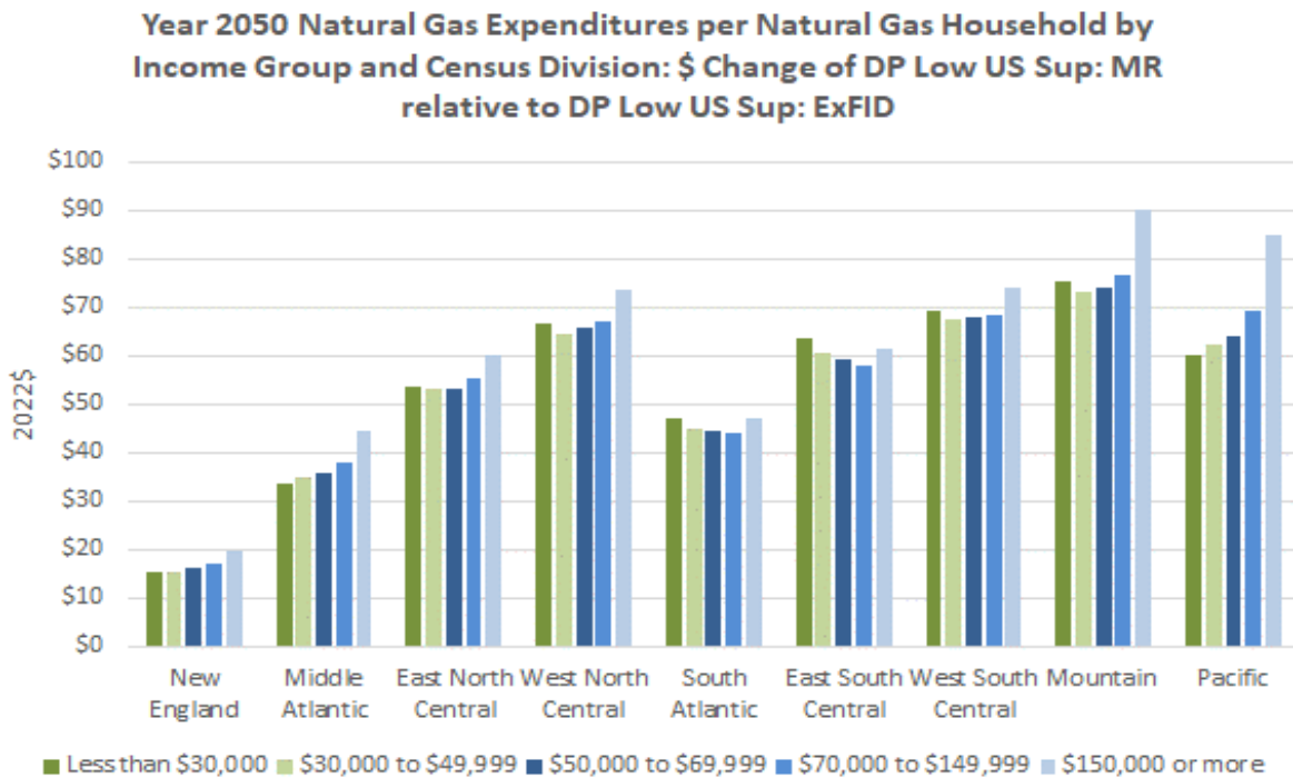
Figure 7. Natural gas expenditure impacts per natural gas household in 2050.
