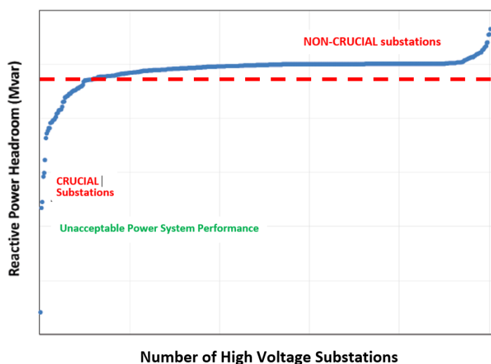
Figure 11: Voltage-based substation cruciality ranking.
