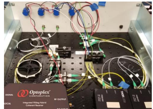
An Optoplex receiver being demonstrated as part of ORNL’s Q-Sens project.
