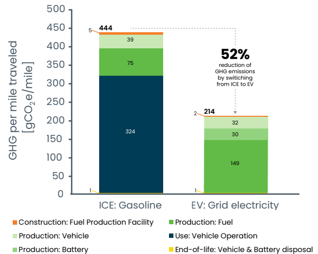
FIGURE 1: Electric vehicles today produce 52% fewer GHGs than their comparable gasoline vehicles on a life cycle basis.
