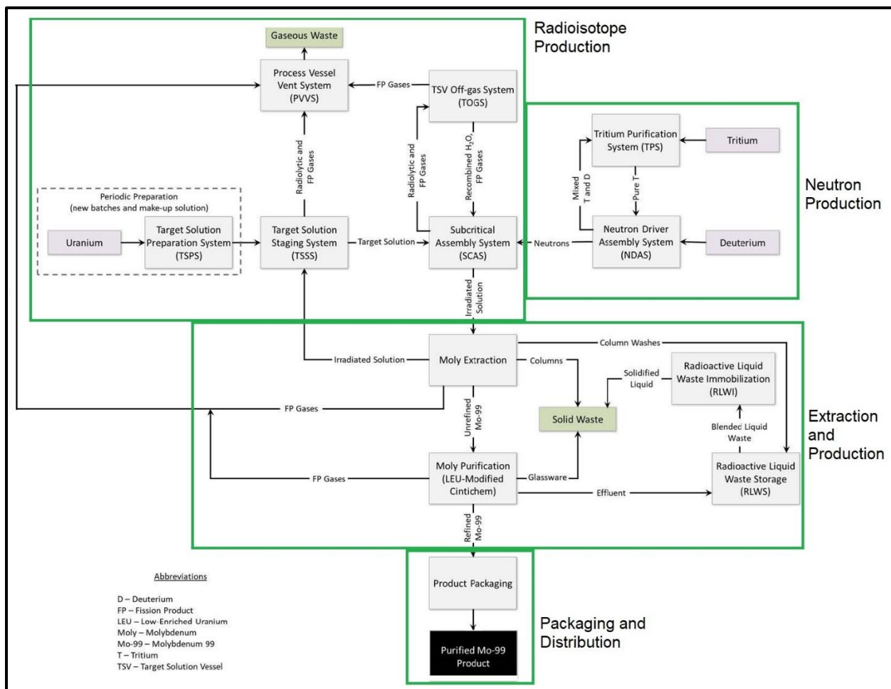
Figure 2-3 Radioisotope Production Process
