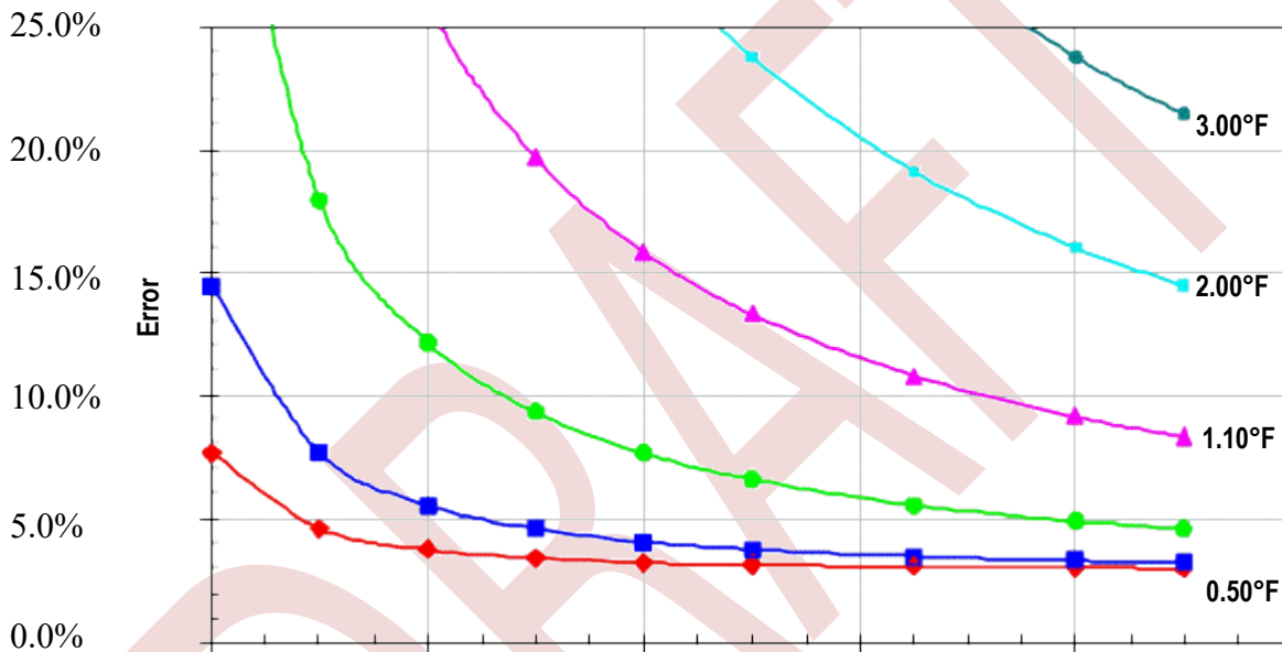
Figure 5-2. Example Influence of Sensor Accuracy on Calculations. 33
