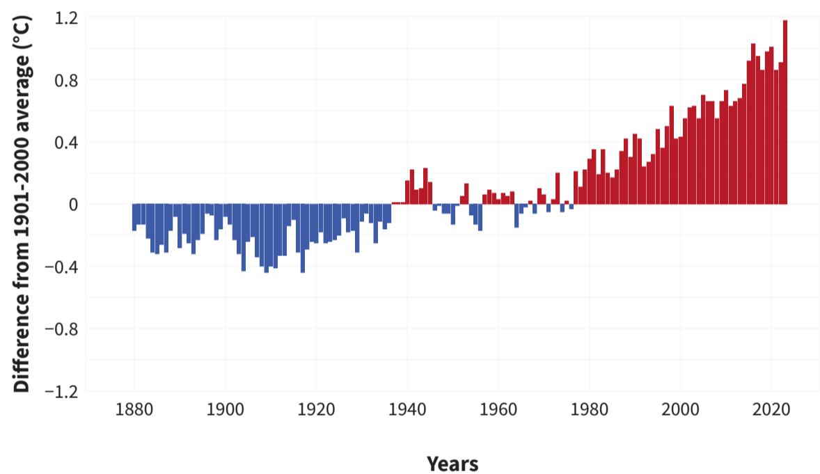
Yearly surface temperature compared to the 20th-century average from 1880–2023. Blue bars indicate cooler-than-average years; red bars show warmer-than-average years. NOAA Climate.gov graph, based on data (https://www.ncdc.noaa.gov/cag/global/time-series) from the National Centers for Environmental Information.
