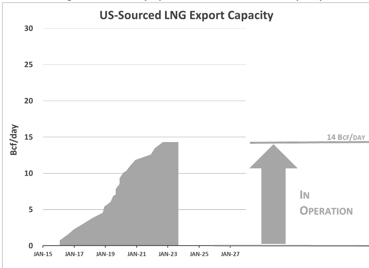
Figure 3 – Currently Operational US-Sourced LNG Capacity
