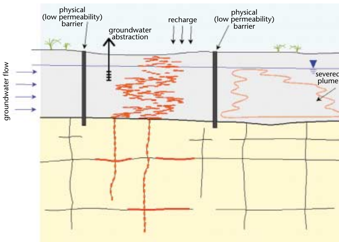
Figure 28 | Physical isolation of DNAPL source zone
