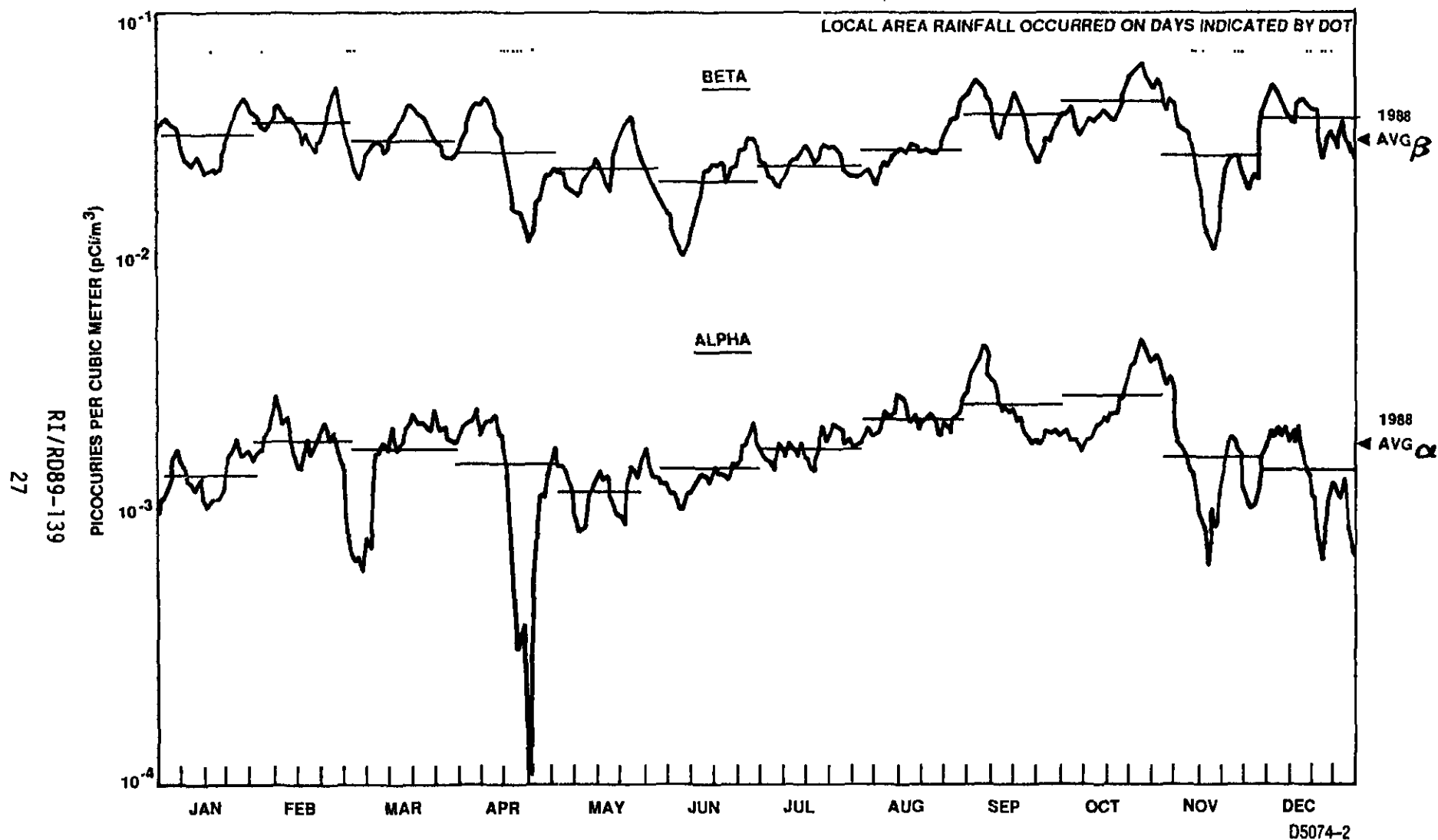
Figure 5. Weekly, Monthly, and Annual Averaged Long-Lived Airborne Radioactivity at the De Soto and Santa Susana Field Laboratories Sites--1988
