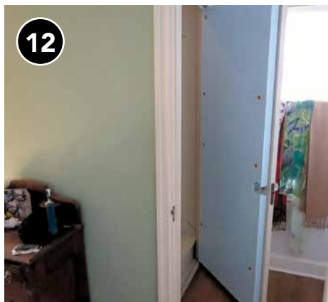
12 Weatherstrip and insulate door using fire safe materials that meet the requirements of the authority having jurisdiction.
