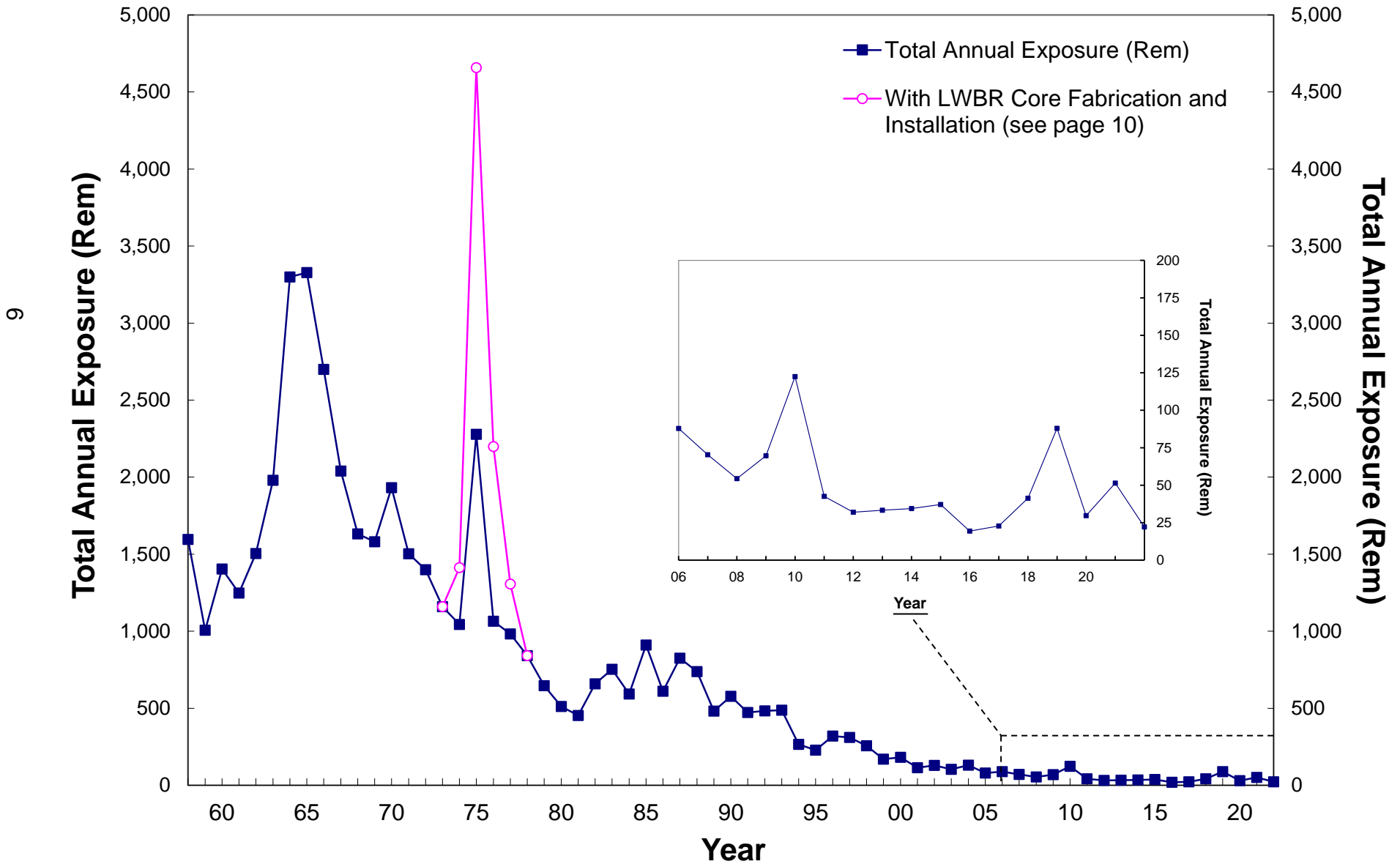
FIGURE 1 TOTAL RADIATION EXPOSURE RECEIVED BY PERSONNEL AT NAVAL REACTORS' DEPARTMENT OF ENERGY FACILITIES 1958 - 2022
