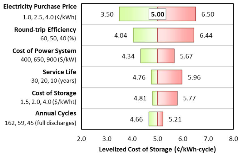
Figure 7(a). Techno-economic scenarios for achieving the $0.05/kWh e LCOS goal using the ARPA-E DAYS formula [3]
