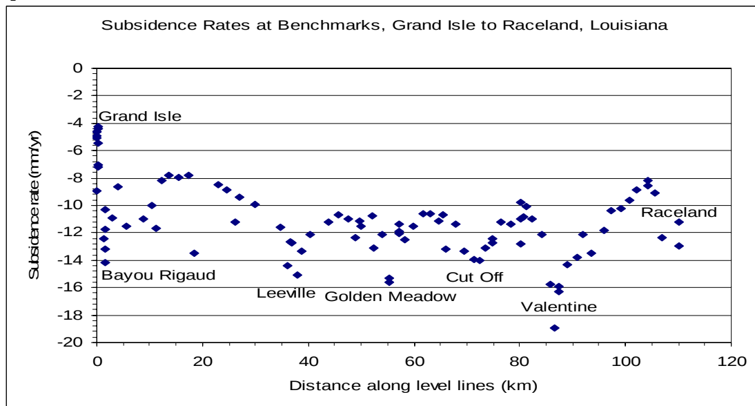
Figure 6. Subsidence rates at benchmarks from 1982 to 1993 interval.
