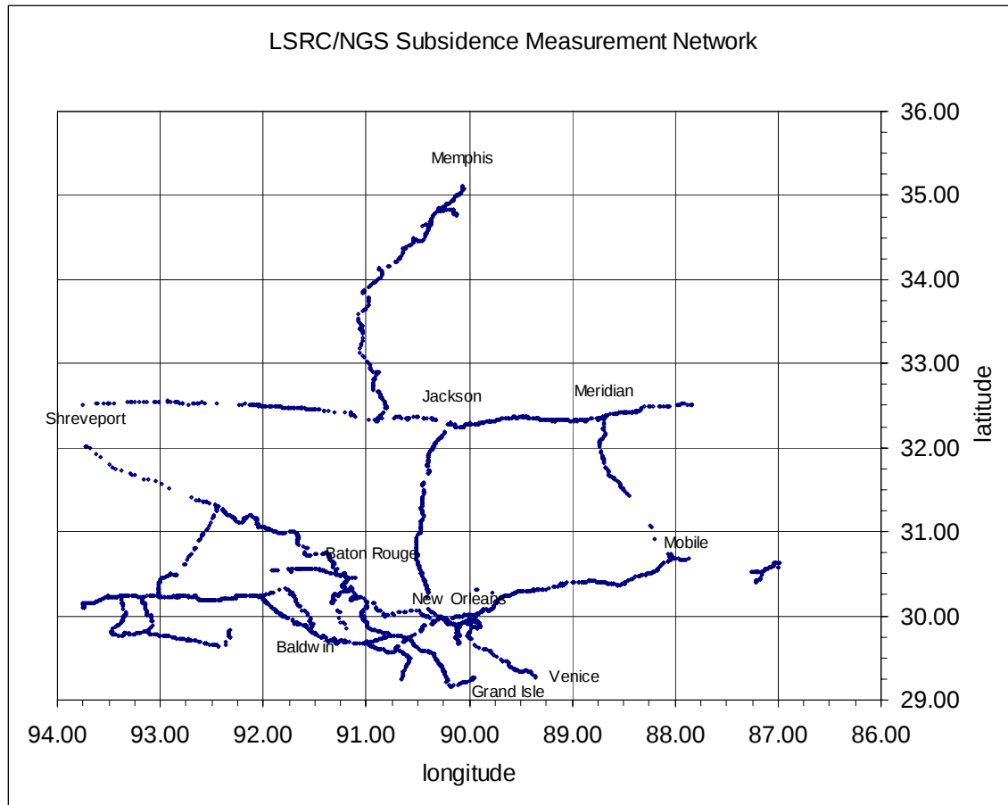
Figure 3. Plot of first-order benchmarks included in the subsidence measurement network.
