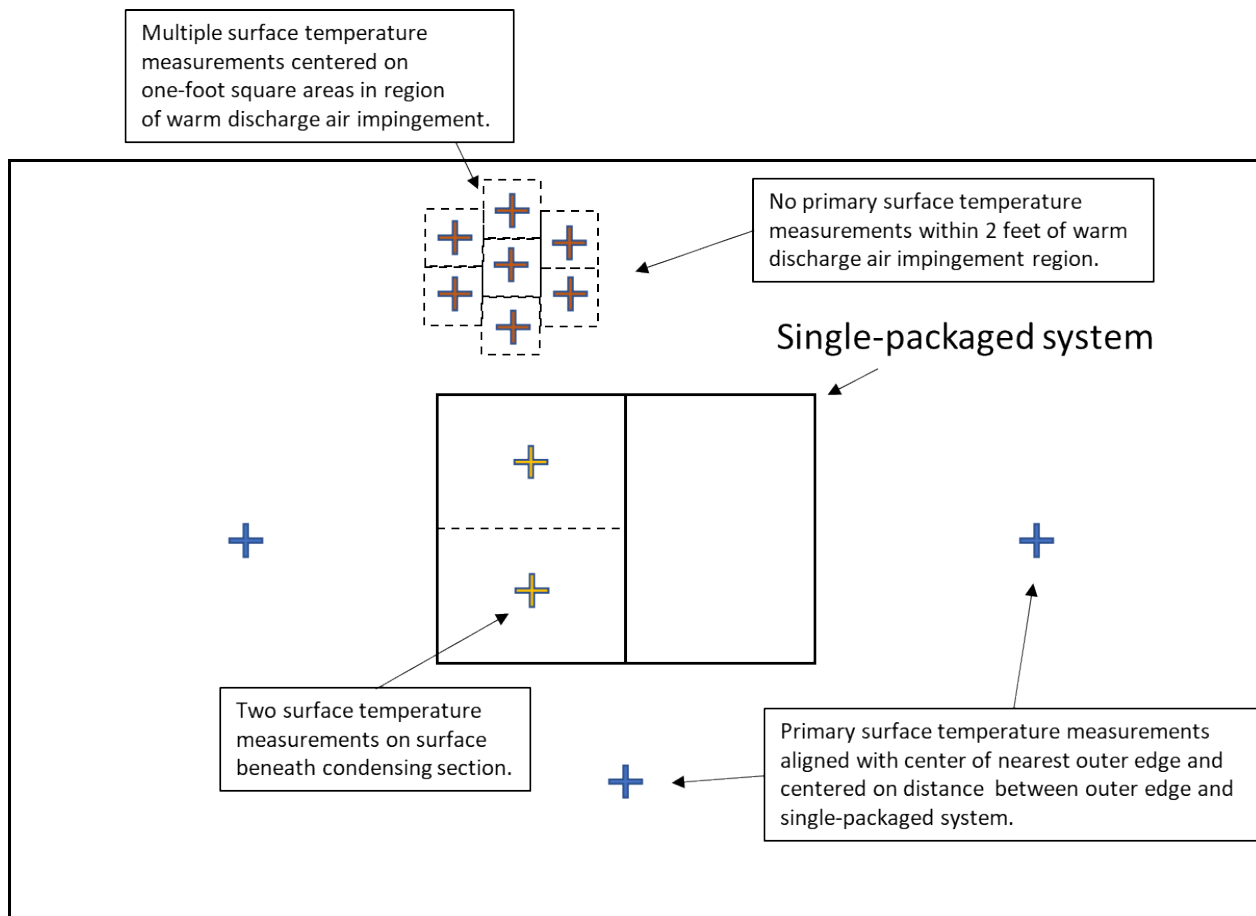
Figure C5: Illustration of Layout of Surface Temperature Sensors on Face of Calibrated Box on which Single-Packaged Dedicated System is Mounted when Using Section 3.5.2.10.2.7 of 10 CFR part 431 Subpart R, Appendix C.
