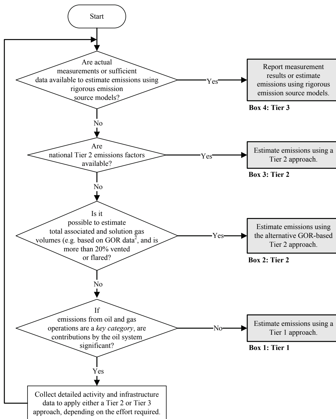
Figure 4.2.2 Decision tree for crude oil production
