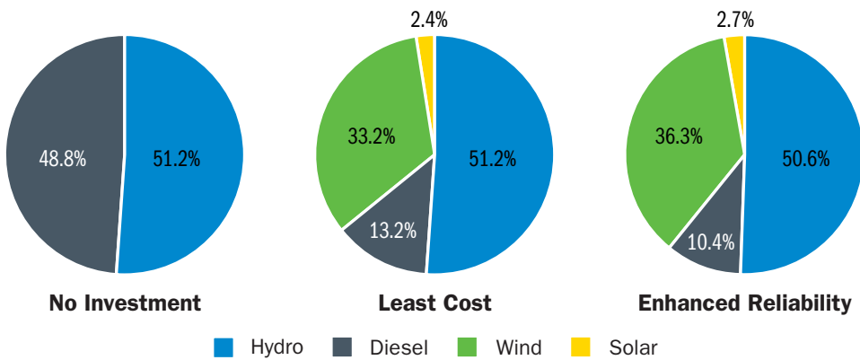
Figure 1. The optimal generation mixes for each of the goal scenarios: no investment, least cost, and enhanced reliability. Illustration by Nicole Leon, National Renewable Energy Laboratory
