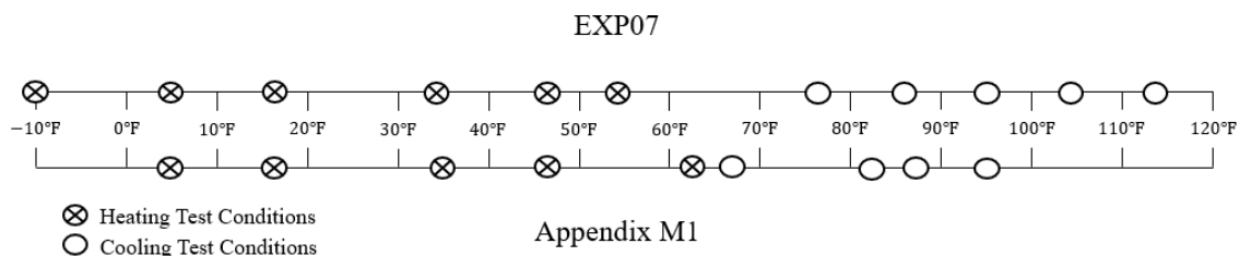
Figure II-1: Comparison of Outdoor Dry-Bulb Temperature Test Conditions between EXP07 and DOE Test Procedure (Appendix M1) for CAC/HPs
