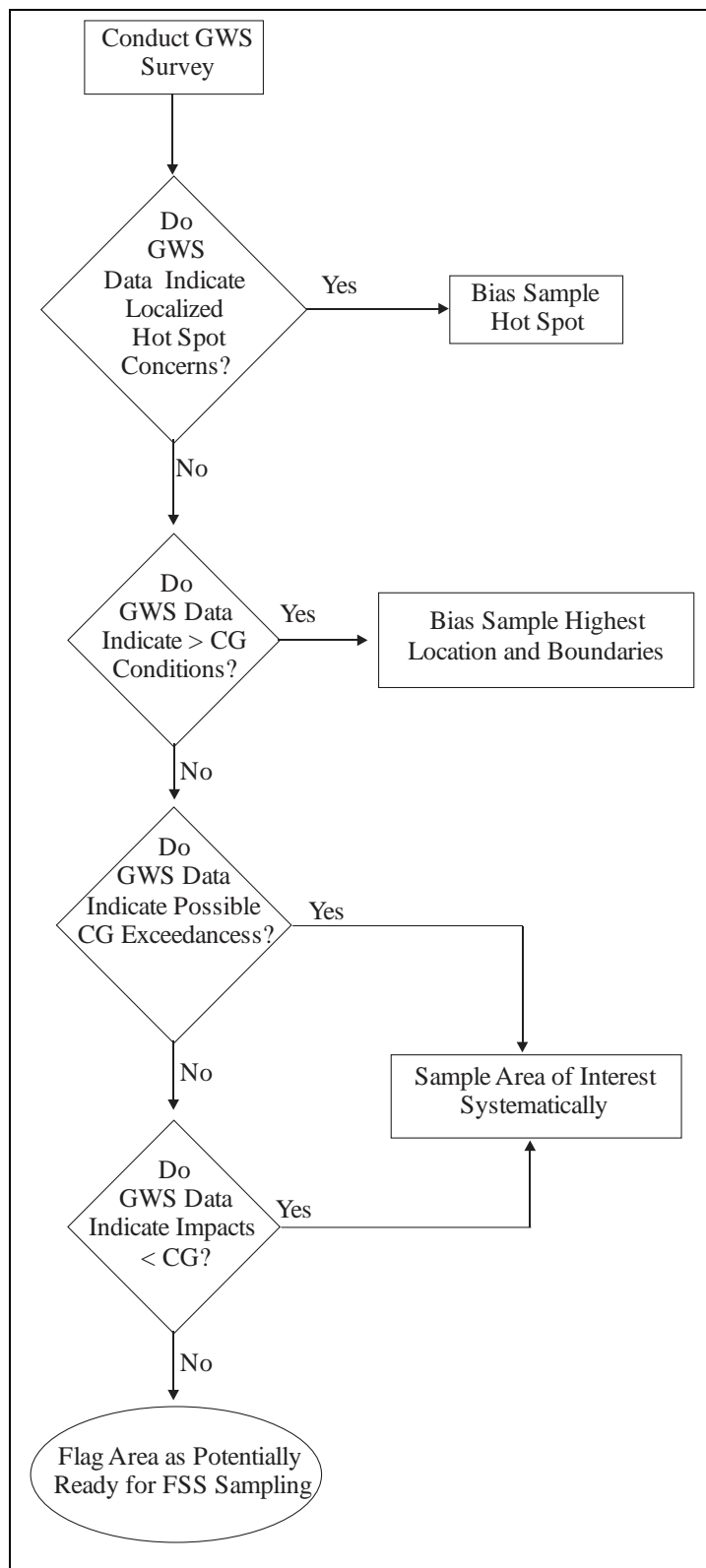
Figure 5 Flowchart Showing Decision-Making Process Based on GWS Data Collection
