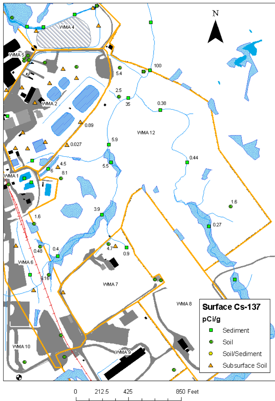
Figure J.9 WMA 12 South Surface Cs-137 Activity Concentrations
