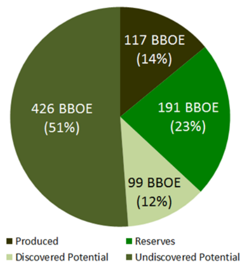
Global Arctic Conventional Endowment
