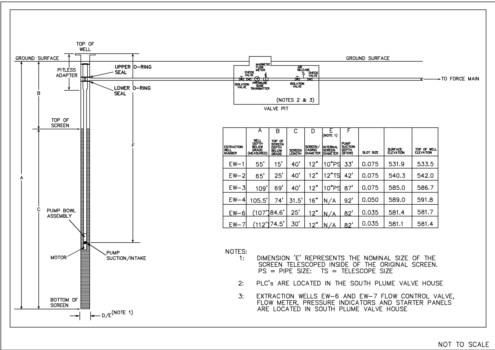
Figure 9. South Plume Module Extraction Well Installation Details
