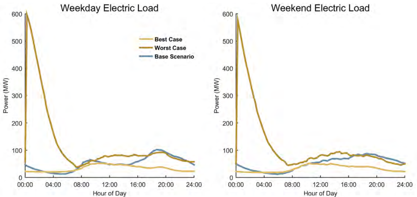
Baseline-, Worst- case, and Best-case load profiles for Aggressive EV adoption for Jacksonville urban area
