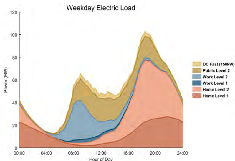
Load Forecasts for Jacksonville under an Aggressive Adoption Scenario
