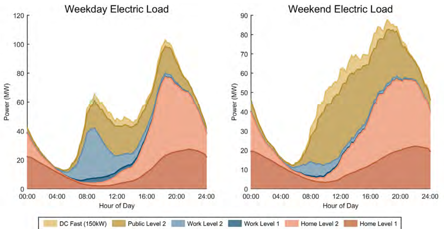
Load Profile for Aggressive EV adoption scenario of Jacksonville urban area
