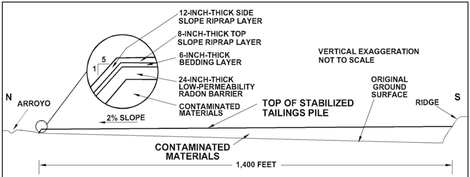
Typical North-South Cross Section of the Mexican Hat Disposal Cell.
