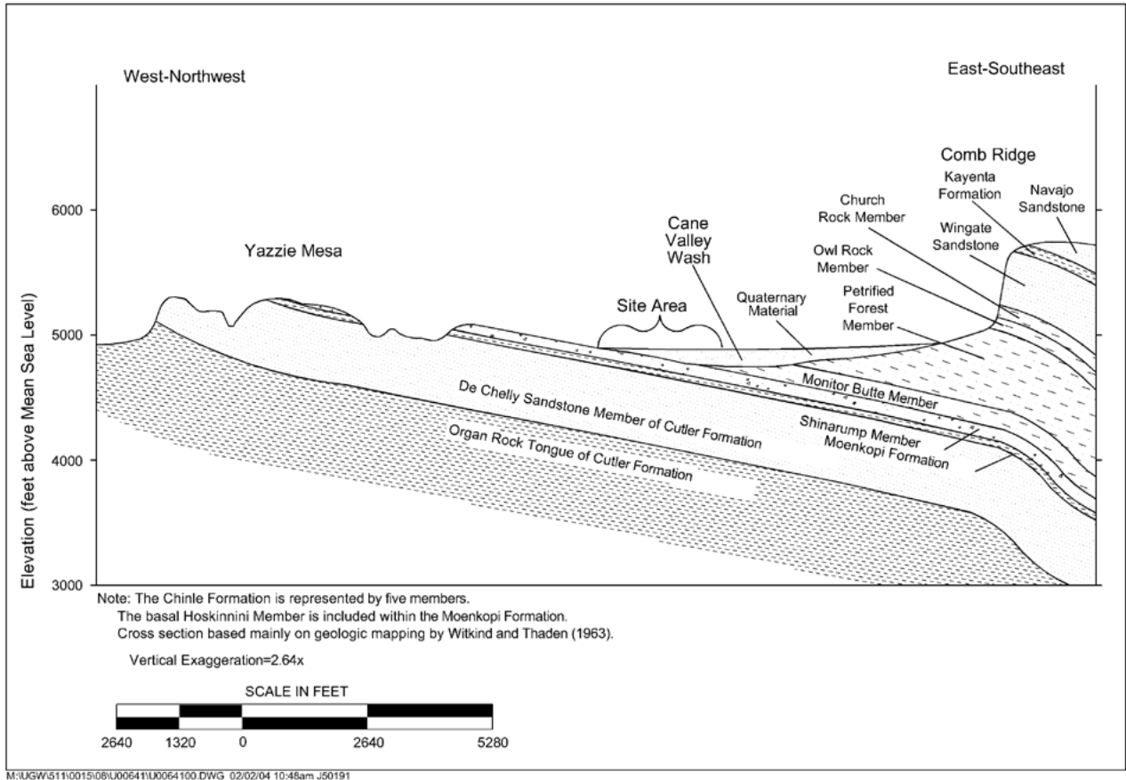
Geologic Features in the Monument Valley Area.
