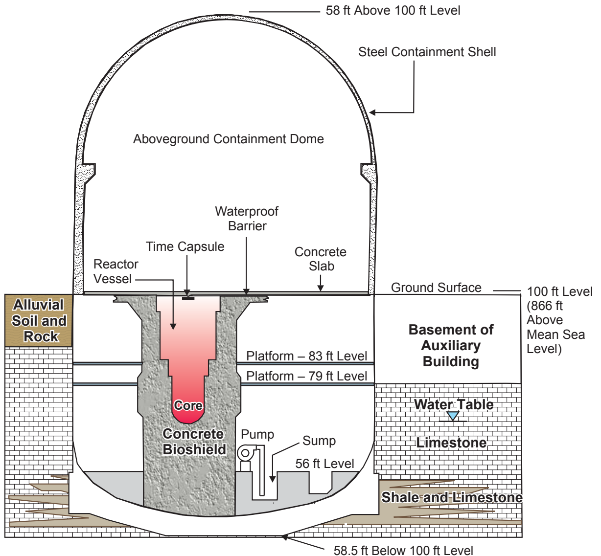
Cross Section of the Piqua Decommissioned Reactor Building.
