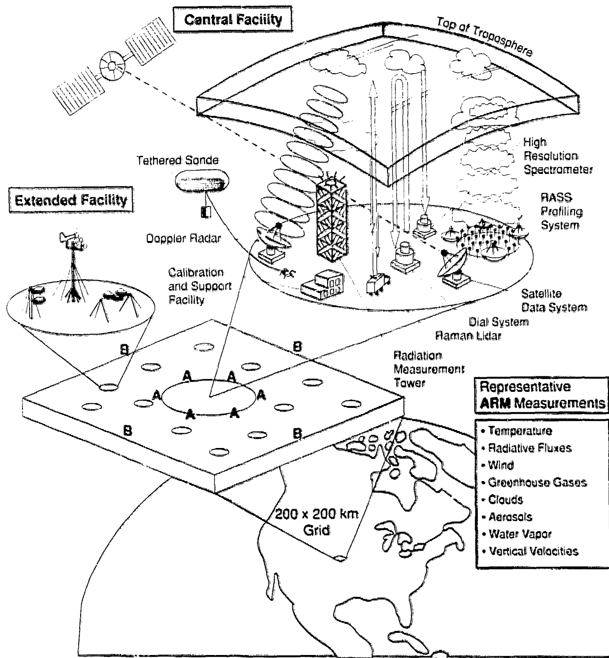
Figure 1.2 General Configuration of the ARM Measurement Grid and Representative Instrumentation for the Central Facility
