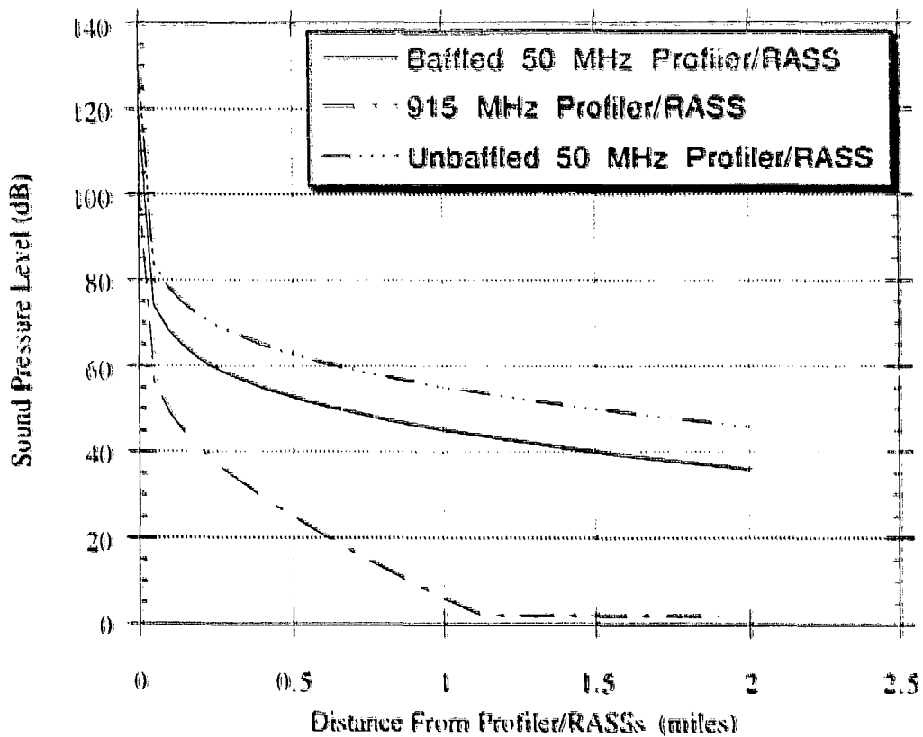
Figure 3.1 Decay of Sound Pressure Level in Distance for the Profiler/RASSs
