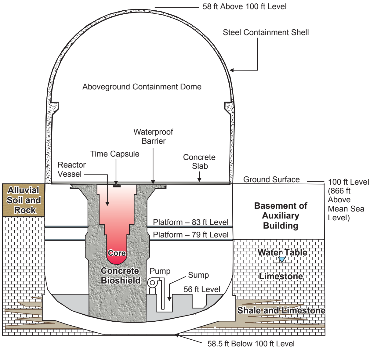
Cross Section of the Piqua Decommissioned Reactor Building.
