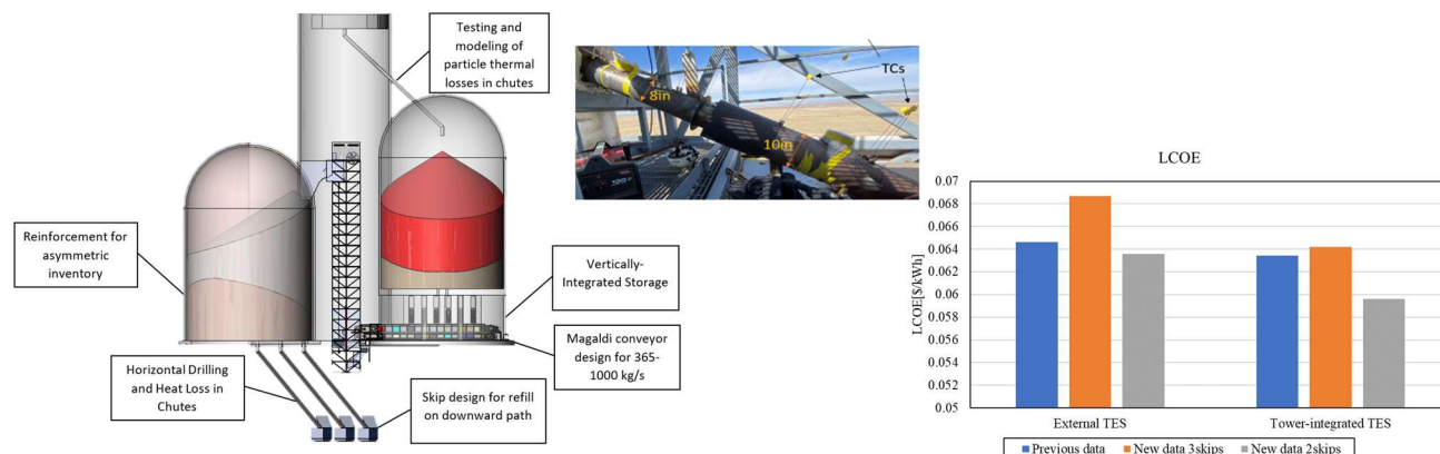
Figure 1. (Left) Primary focus areas of HOTPAC; (Mid) Instrumented chute; (Right) LCOE Results
