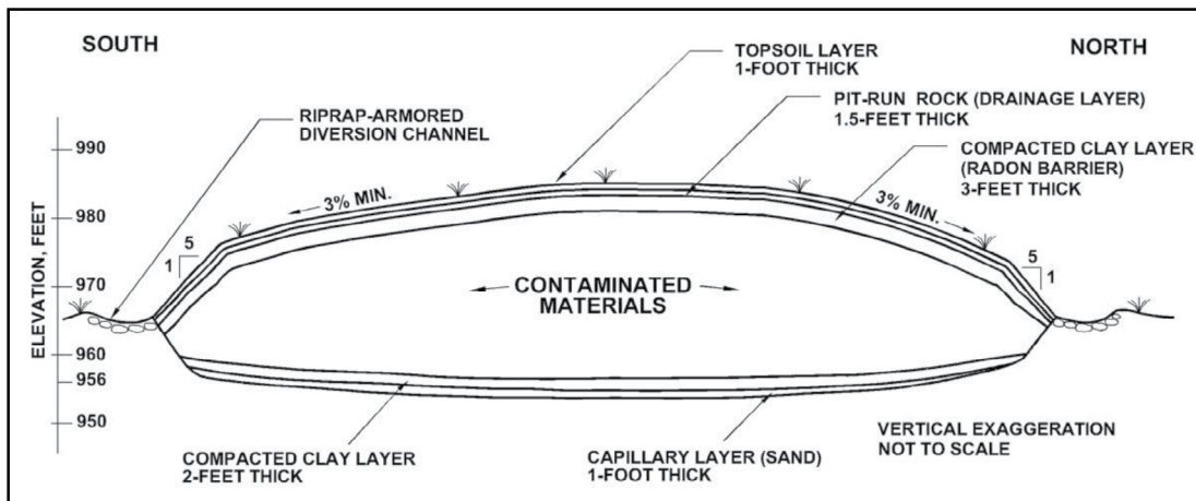
South-North Cross Section of Canonsburg Disposal Cell.
