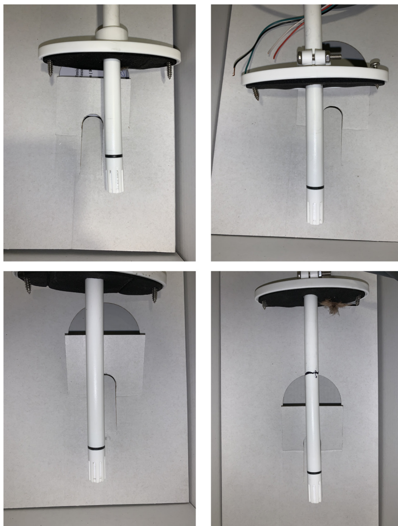
Figure 28. Photos of each of the X_2 duct probes from test homes 1–4 (clockwise, from top left)
