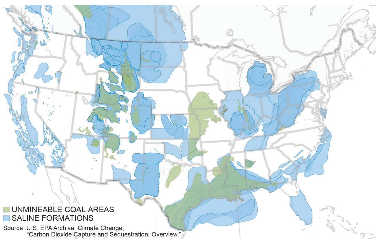
Figure 1-15. U.S. Assessment of Geologic CO 2 Storage Potential
