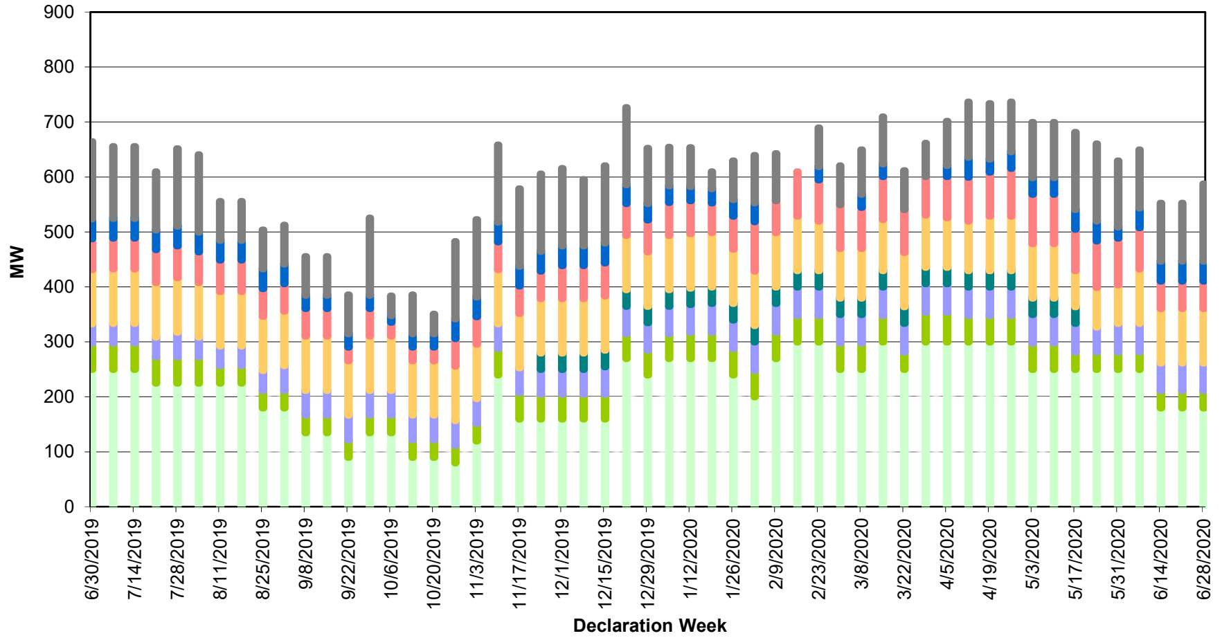
Cumberland System Capacity by Project (Contract Year 2020)
