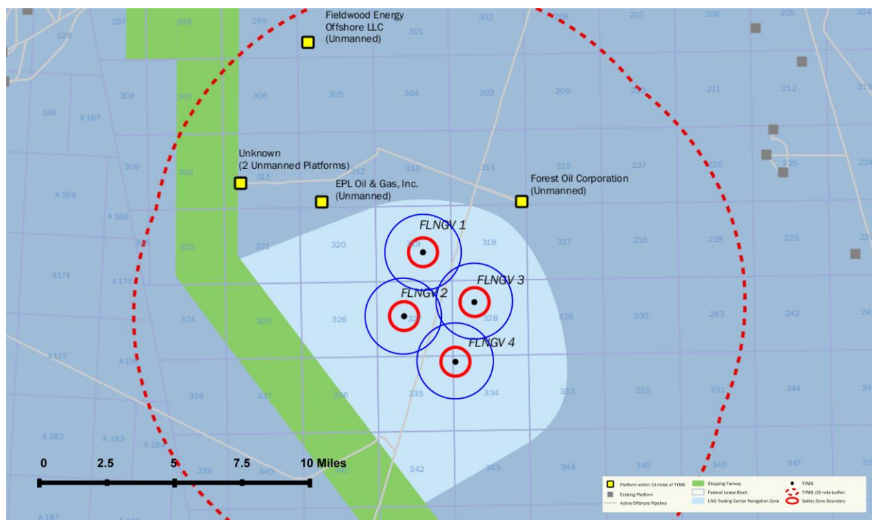
Figure 7: LFL effect zone (in blue) for accidental 2m³ single-tank breach from the FLNGVs
