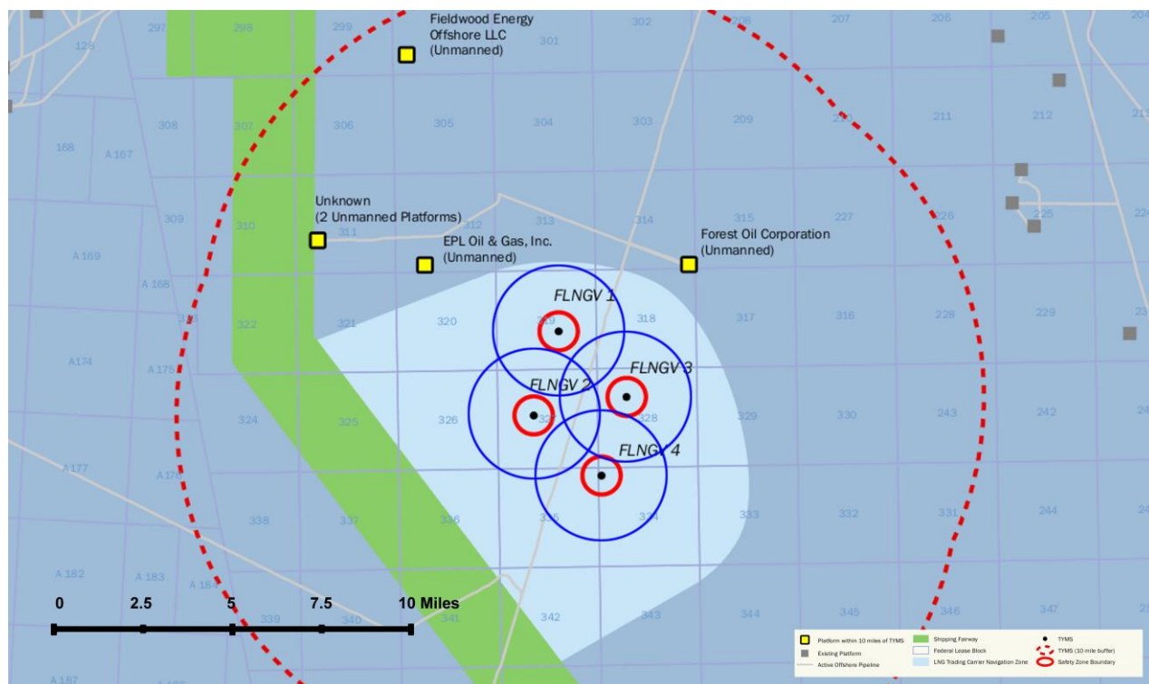
Figure 12: Effect zone (in blue) for 5 kW/m 2 radiation contour from a pool fire caused by cascading event leading to a 12-m 2 breach in three tanks of the FLNGVs
