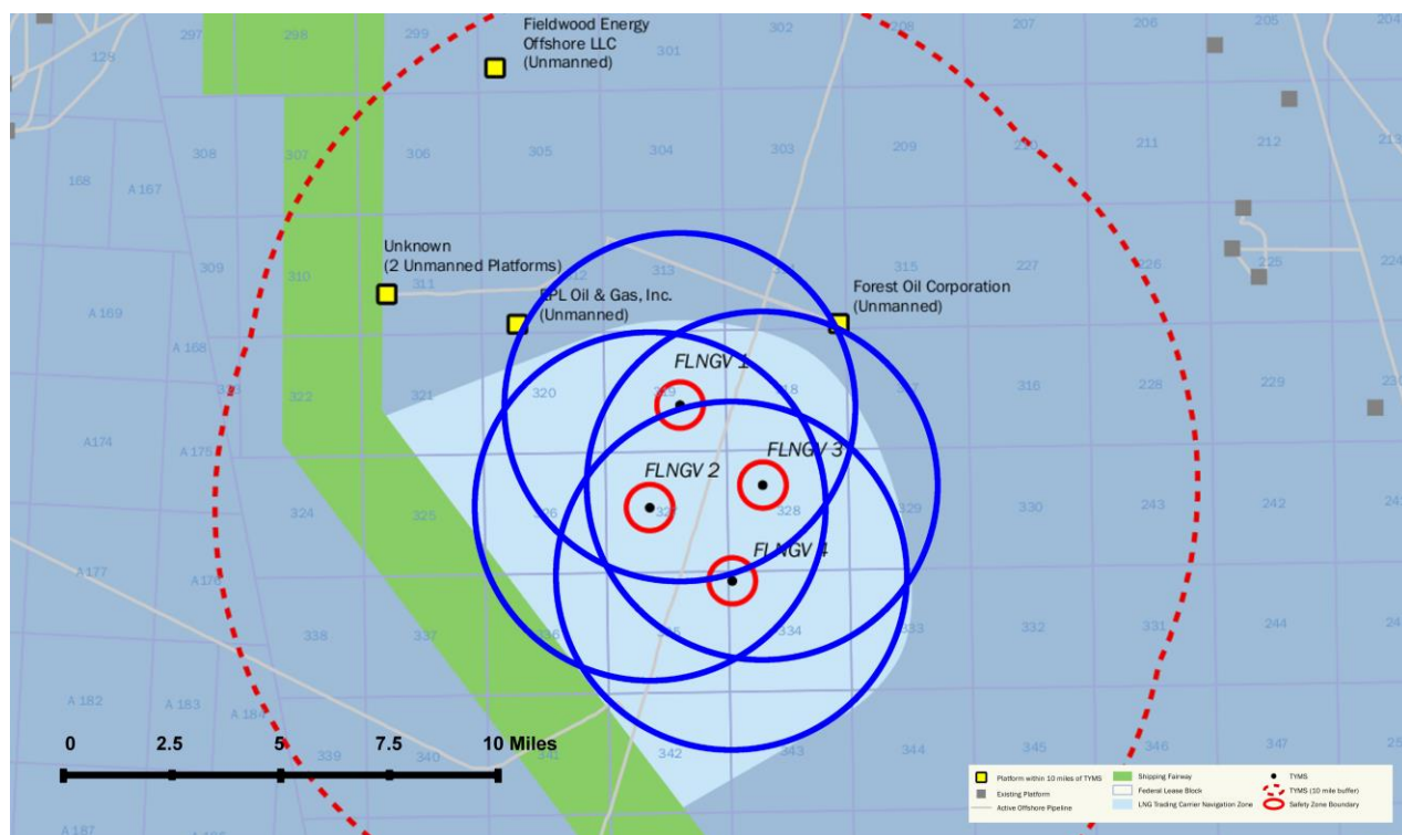
Figure 9: LFL effect zones (in blue) for cascading 12m 3 three-tank breach from the FLNGVs
