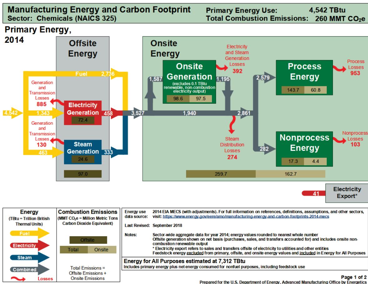
Figure 2. Primary energy use and total GHG combustion emissions for the chemicals sector
