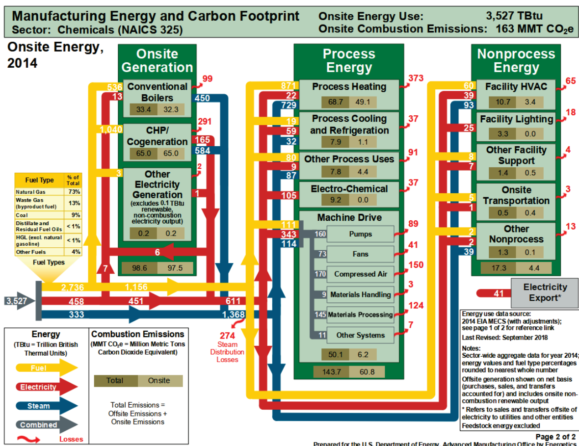
Figure 3. Onsite energy and GHG combustion emissions for the chemicals sector
