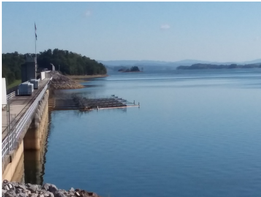
Nine Surface Mixers at Cherokee Dam (Closer View)
