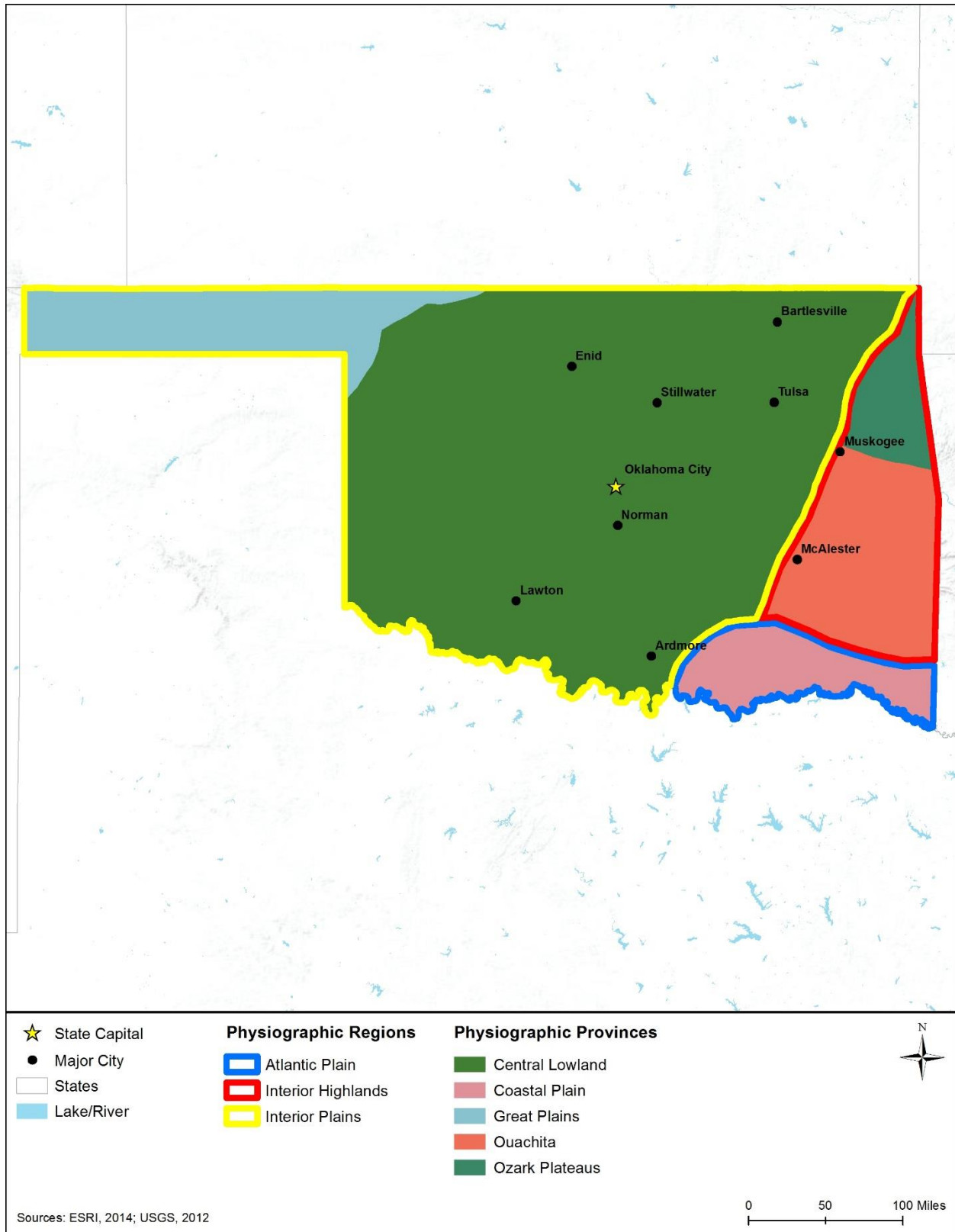
Figure 12.1.3-1: Physiographic Regions and Provinces of Oklahoma
