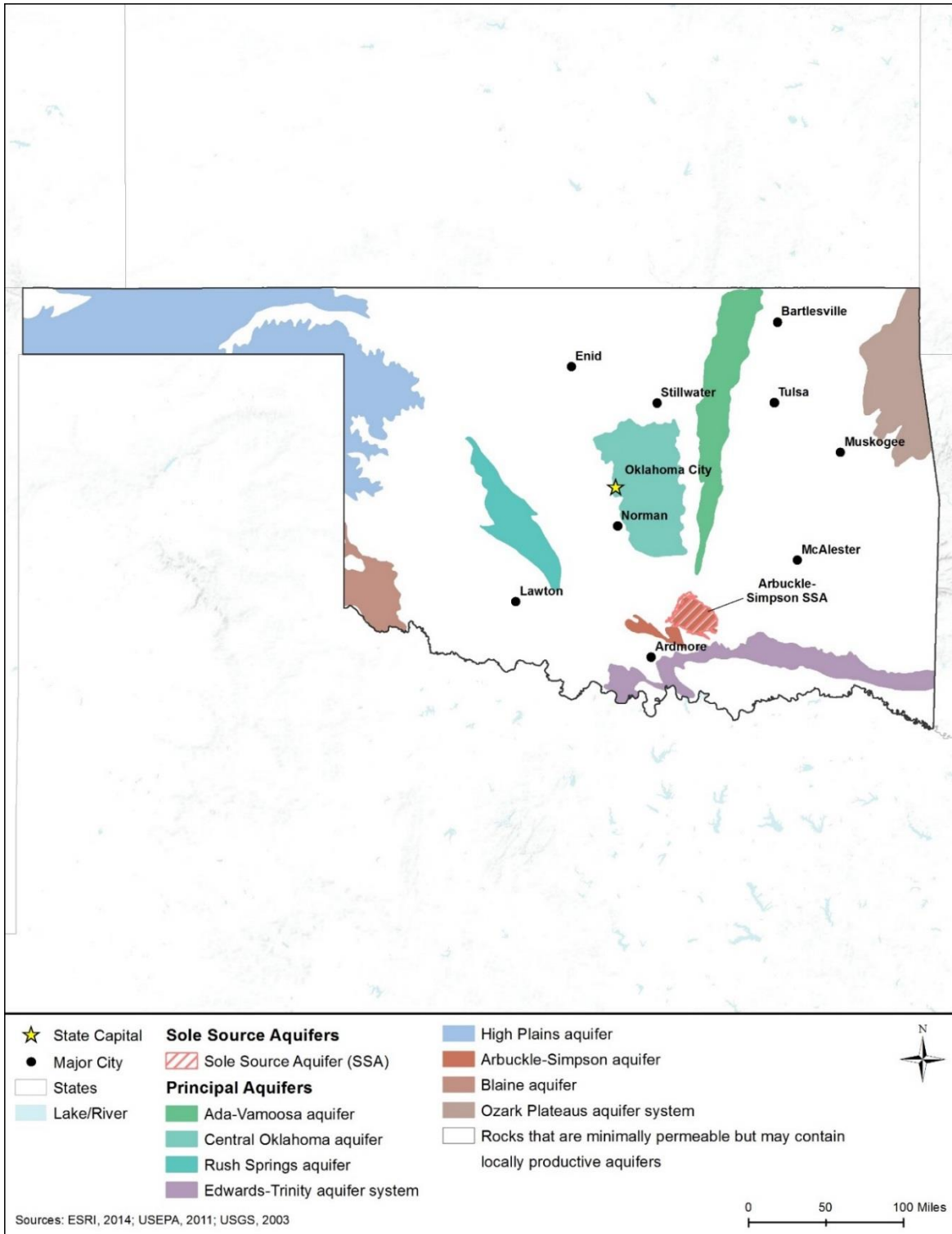
Figure 12.1.4-3: Principal and Sole Source Aquifers of Oklahoma
