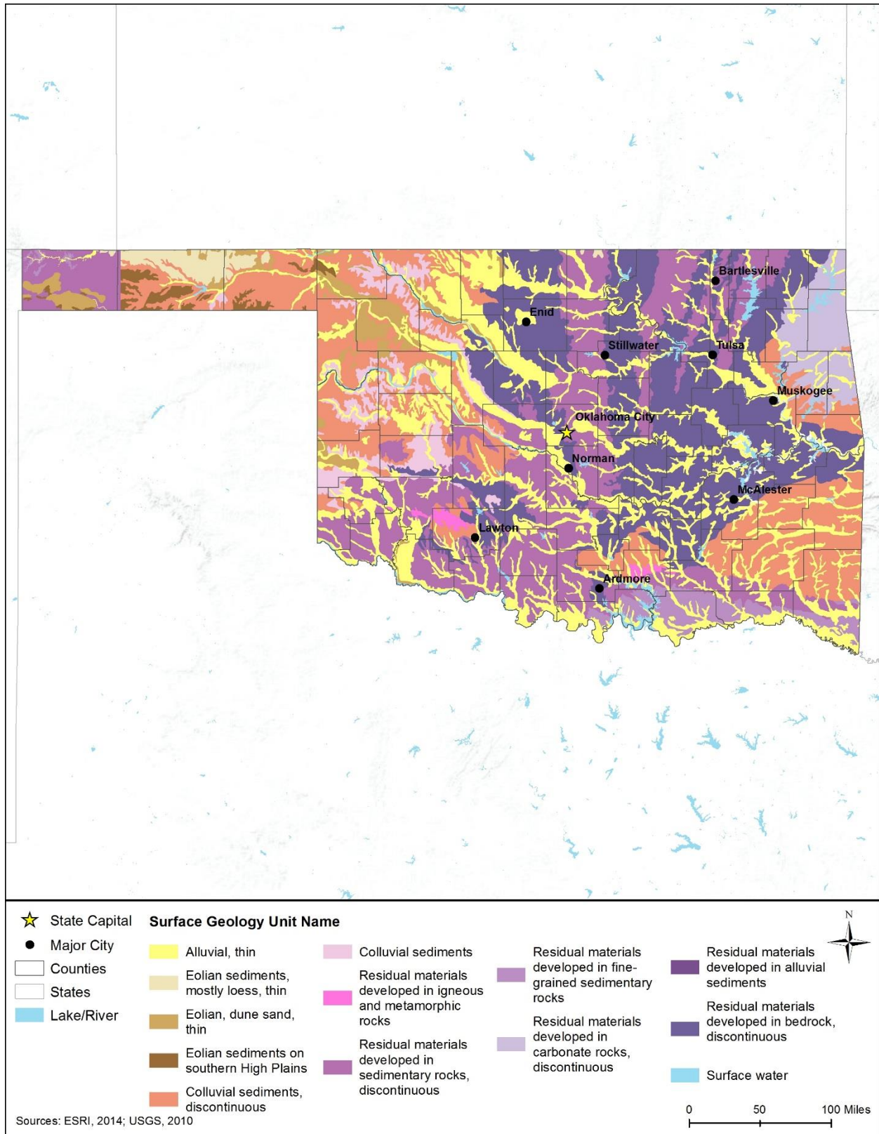
Figure 12.1.3-2: Generalized Surface Geology for Oklahoma
