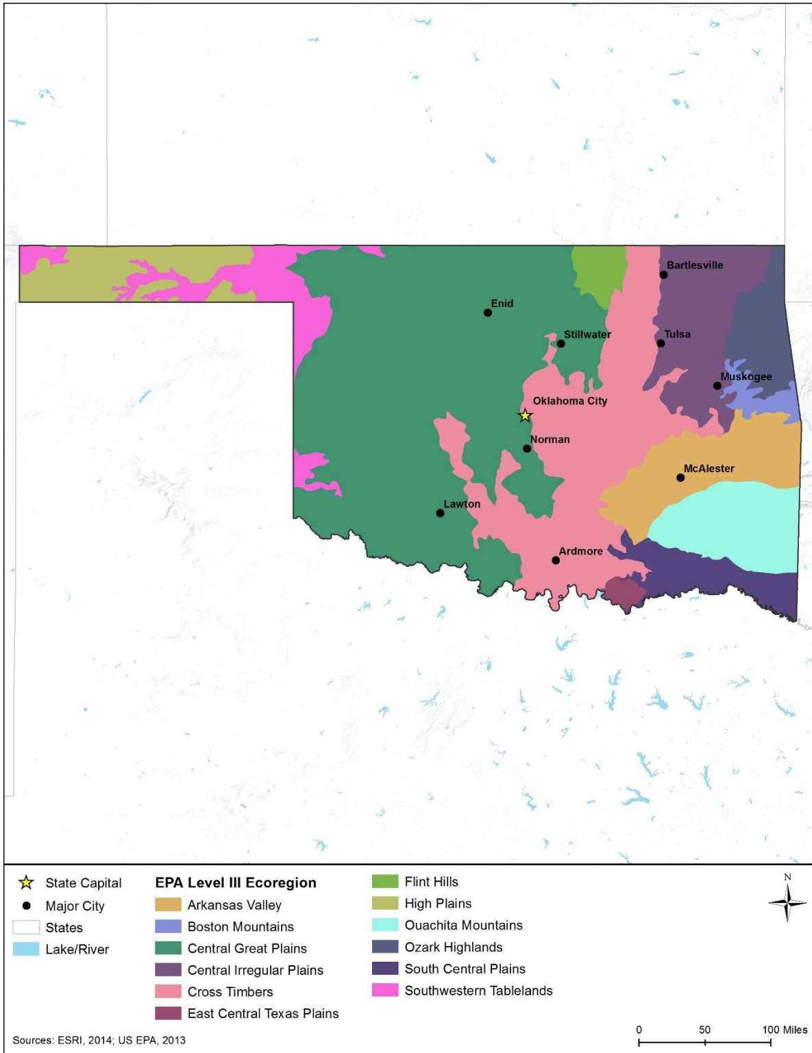
Figure 12.1.6-1. USEPA Level III Ecoregions in Oklahoma
