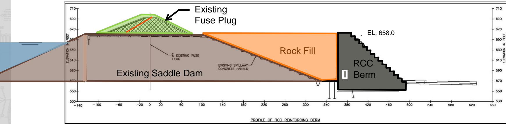
Section View
