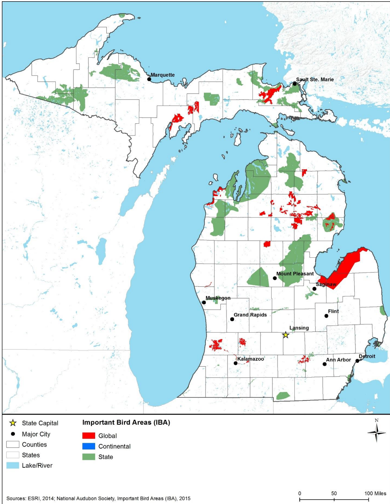
Figure 8.1.6-2: Important Bird Areas in Michigan
