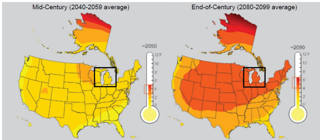
Figure 8.2.14-1: Michigan Low Emission Scenario Projected Temperature Change
