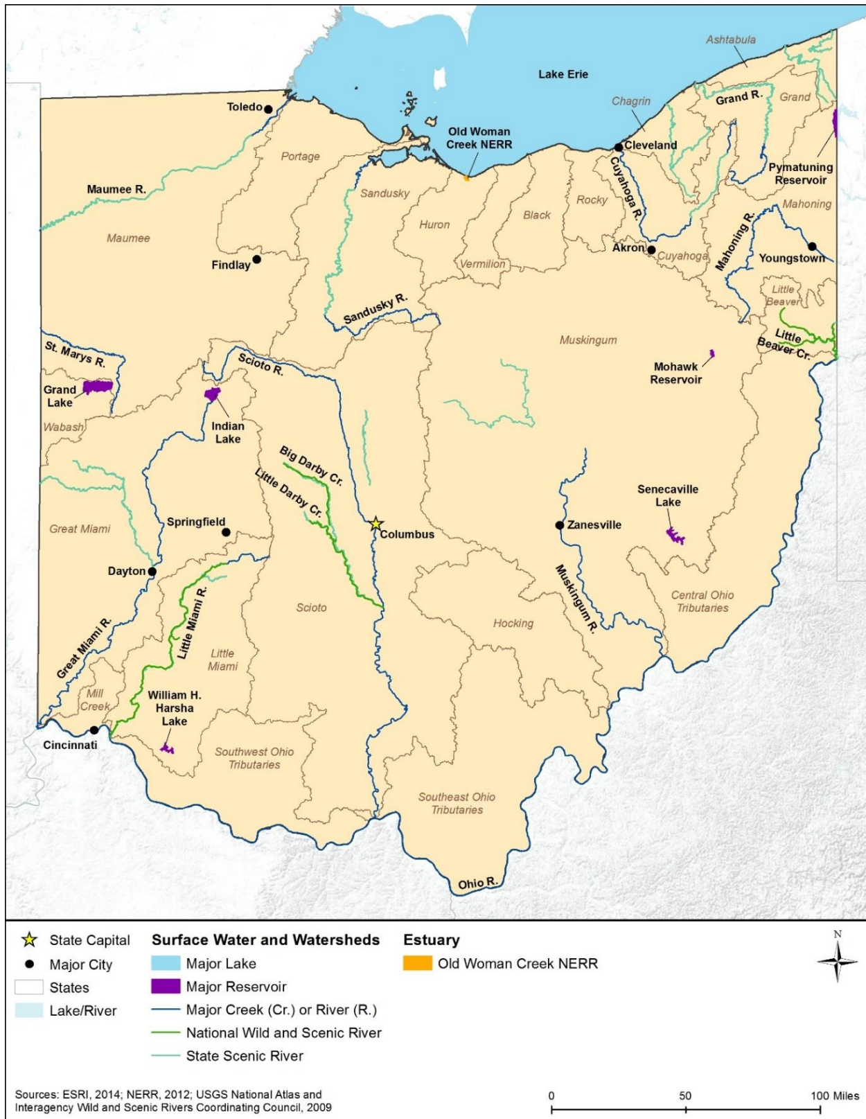
Figure 14.1.4-1: Major Ohio Watersheds and Surface Waterbodies
